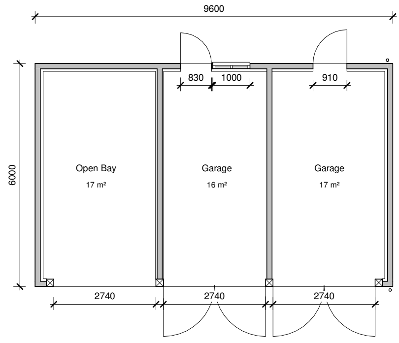
GA Ground Floor Plan As Proposed 1 : 100
