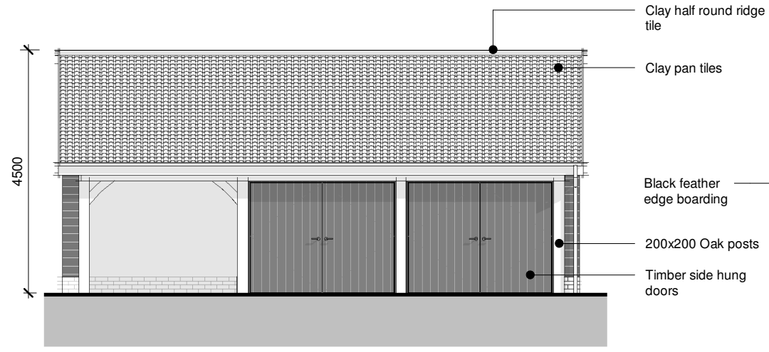
North Elevation As Proposed 1 : 100
