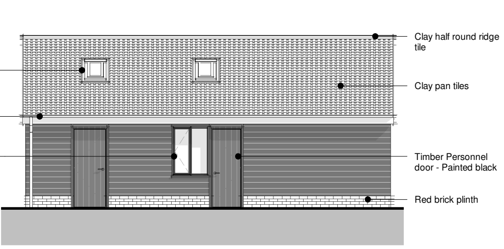
South Elevation As Proposed 1 : 100
