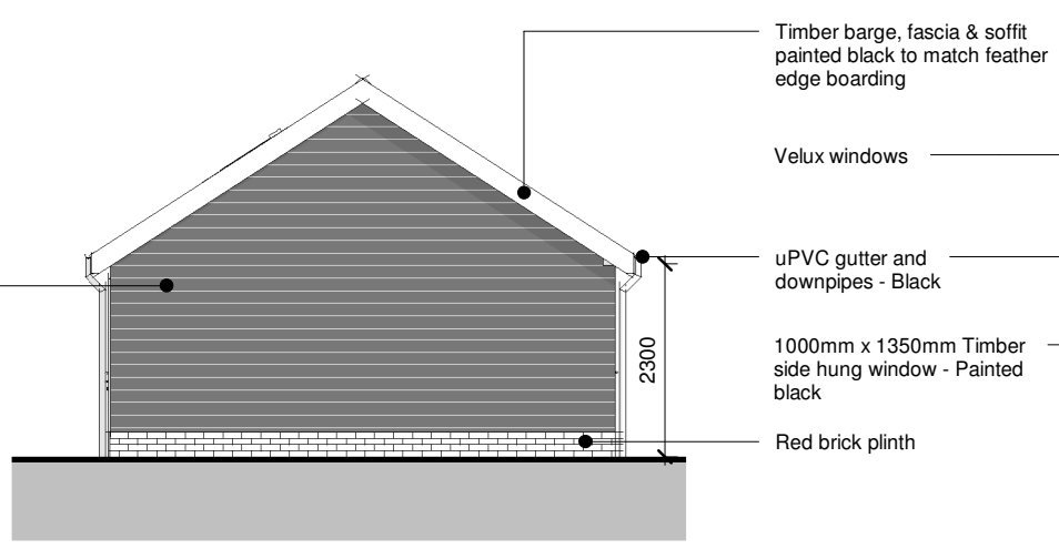
East Elevation As Proposed 1 : 100
