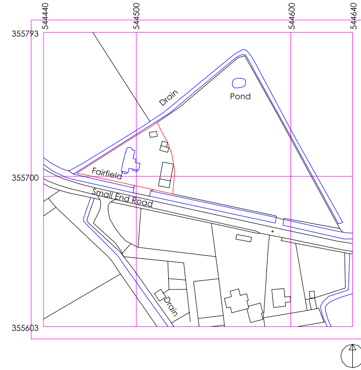
3 Location Plan Ex 1 : 1250
