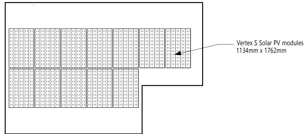
Roof Plan
