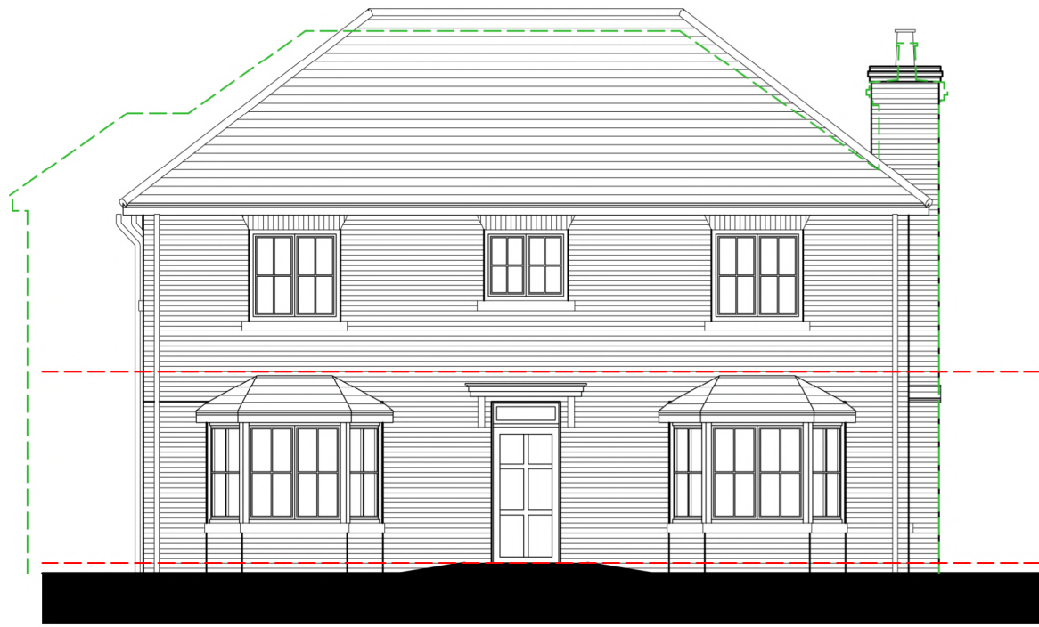
Proposed North Elevation (Front) Scale: 1:100
