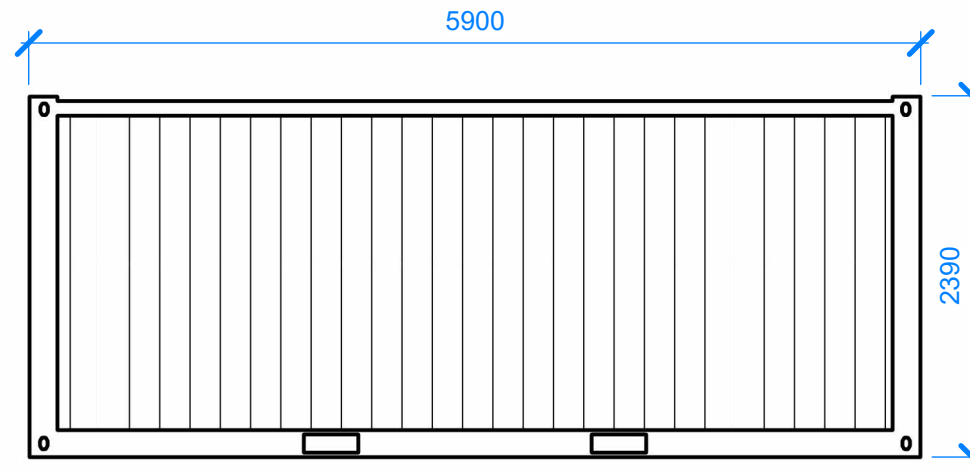
4 Container Elevation - Side 1 : 50
