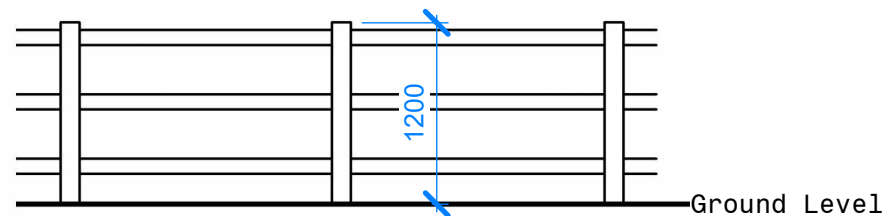
6 Post and Rail Fencing Elevation 1 : 50
