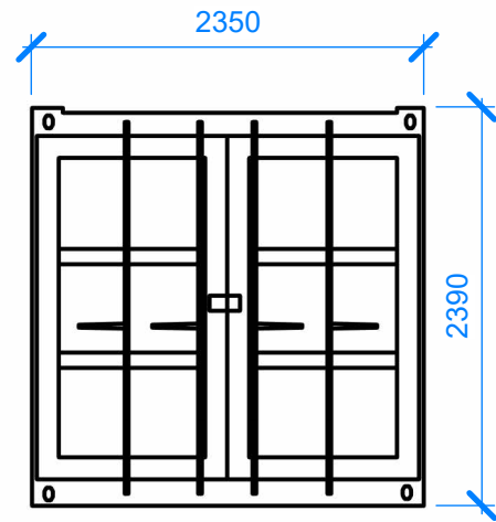
2 Container Elevation - Front 1 : 50
