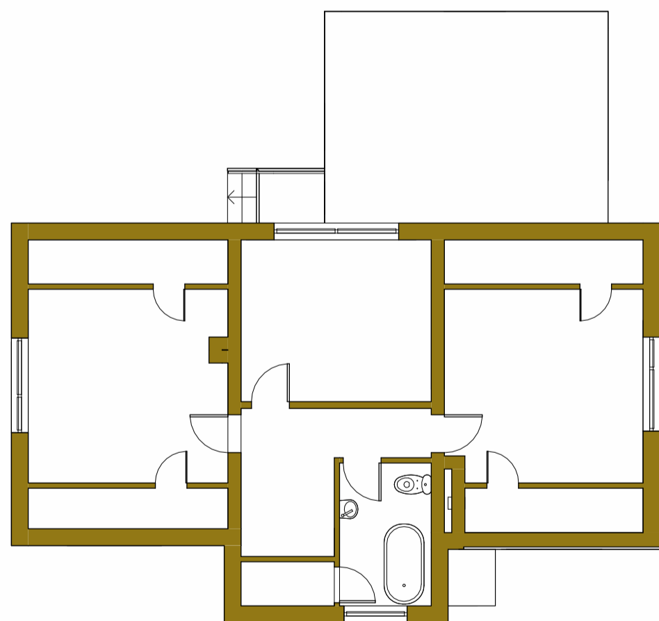
1 Existing Ground Floor 01 1 : 100
