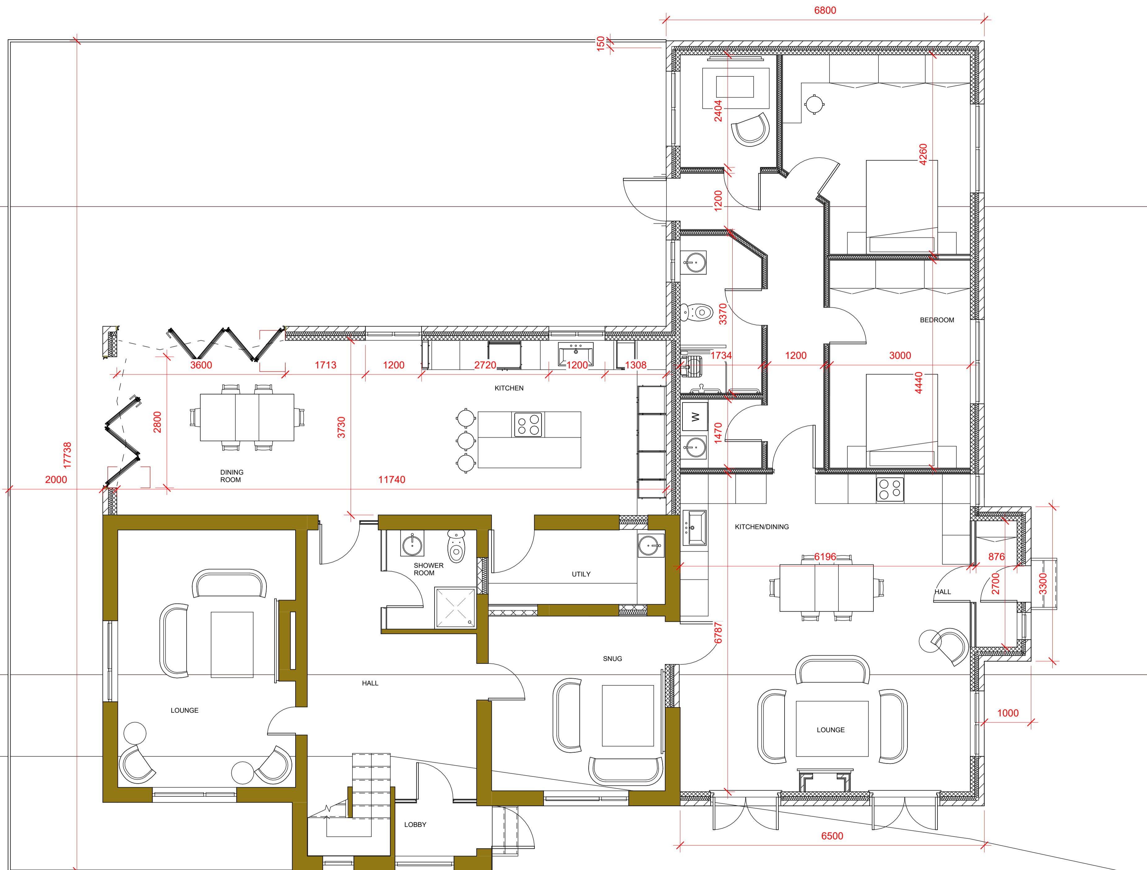
1 Proposed Ground Floor 01 1 : 50
