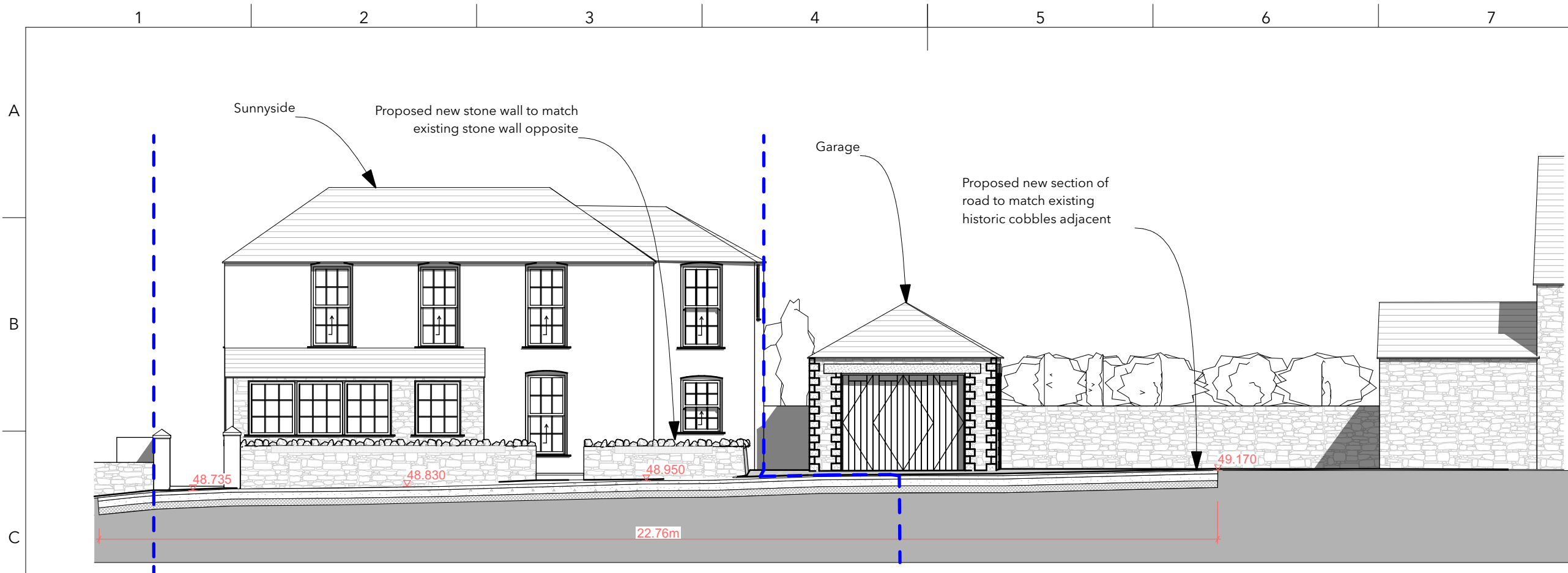
0m 5m 1 Proposed South Elevation 1:100
