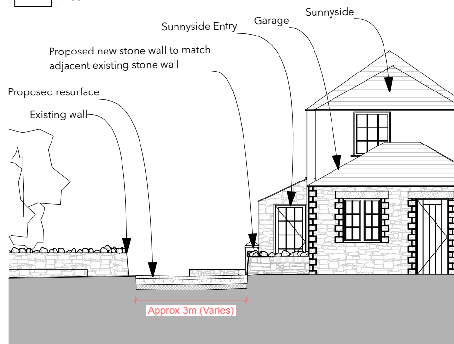
0m 5m 2 Proposed East Elevation 1:100
