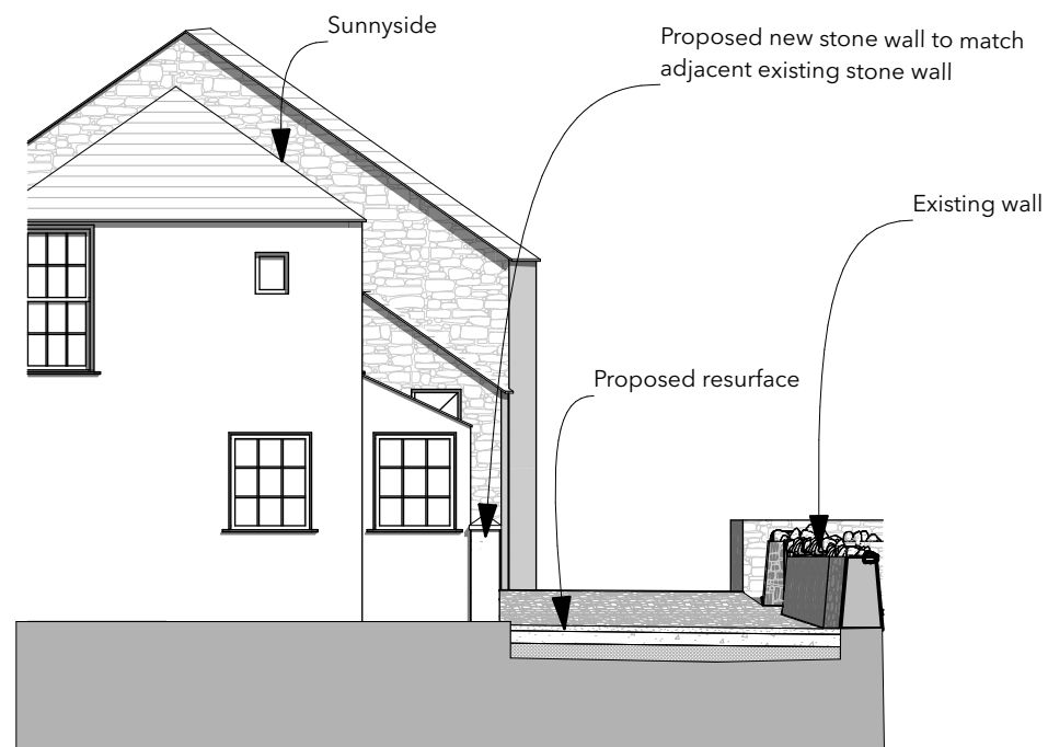
0m 5m 3 Proposed West Elevation 1:100
