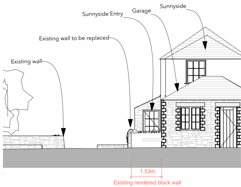
0m 5m 2 Existing East Elevation 1:100
