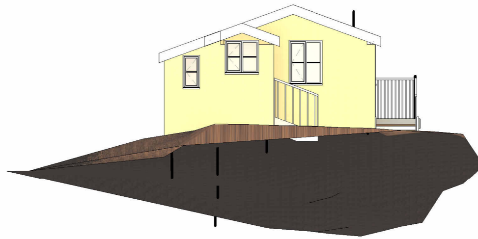
2 North elevation 1 : 100
