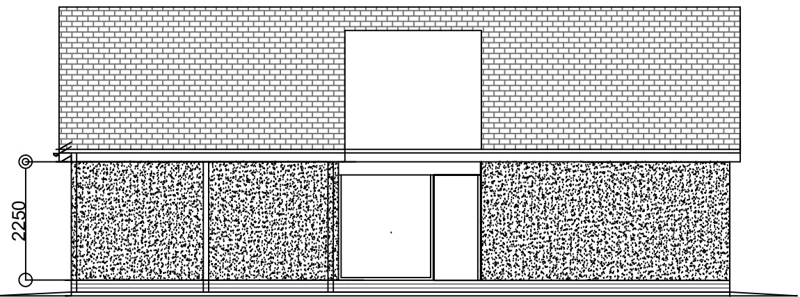
existing elevation to south - to boundary
