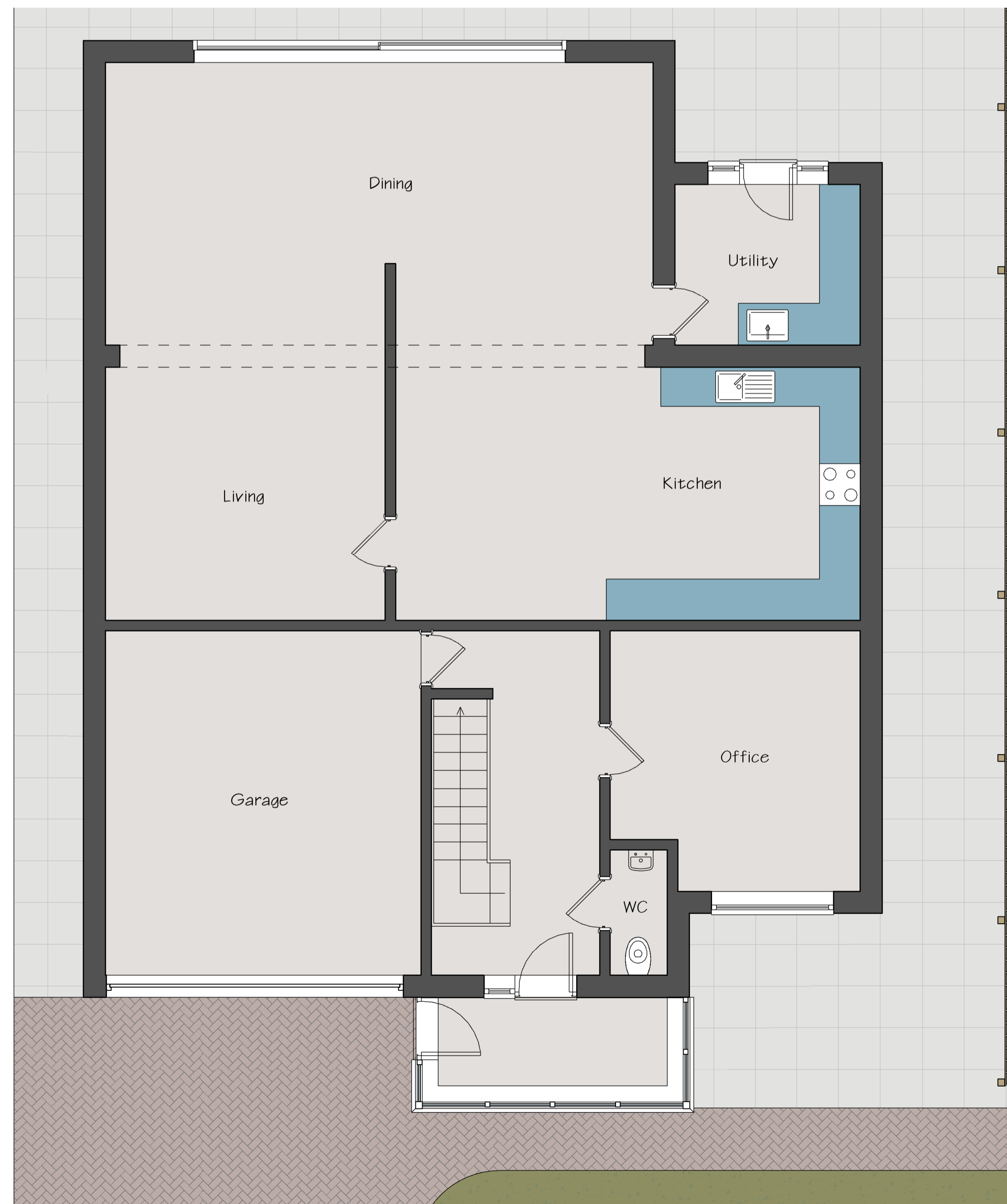
② Existing Ground Floor 1:50
