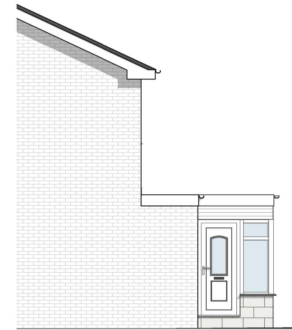
⑦ Existing Elevation Facing South East 1:50
