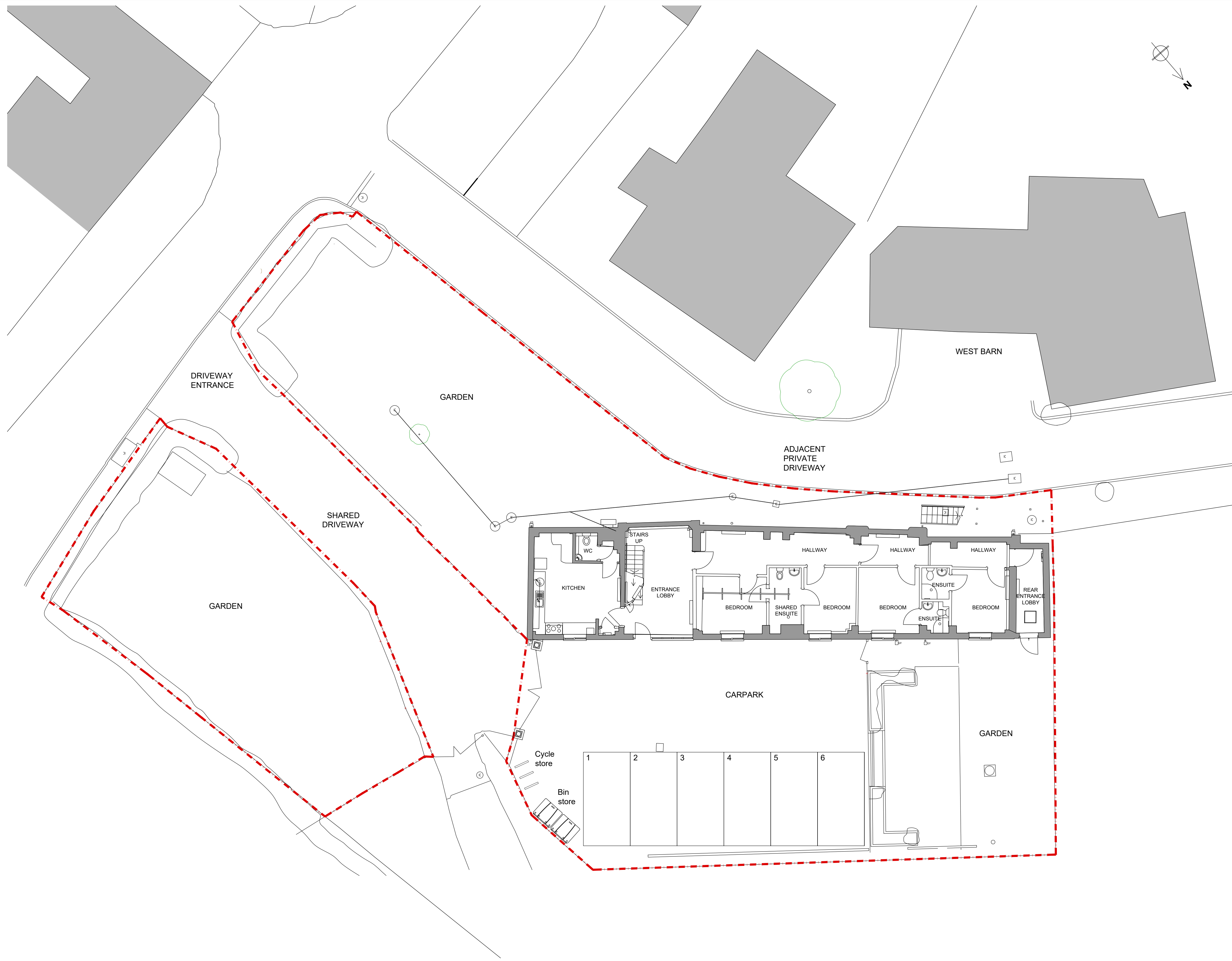
EXISTING SITE AND PROPOSED SITE LAYOUT PLAN
