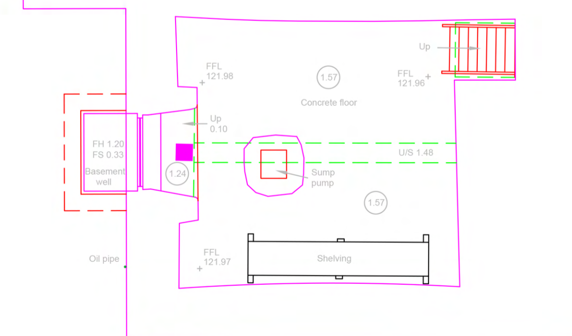
BASEMENT PLAN
