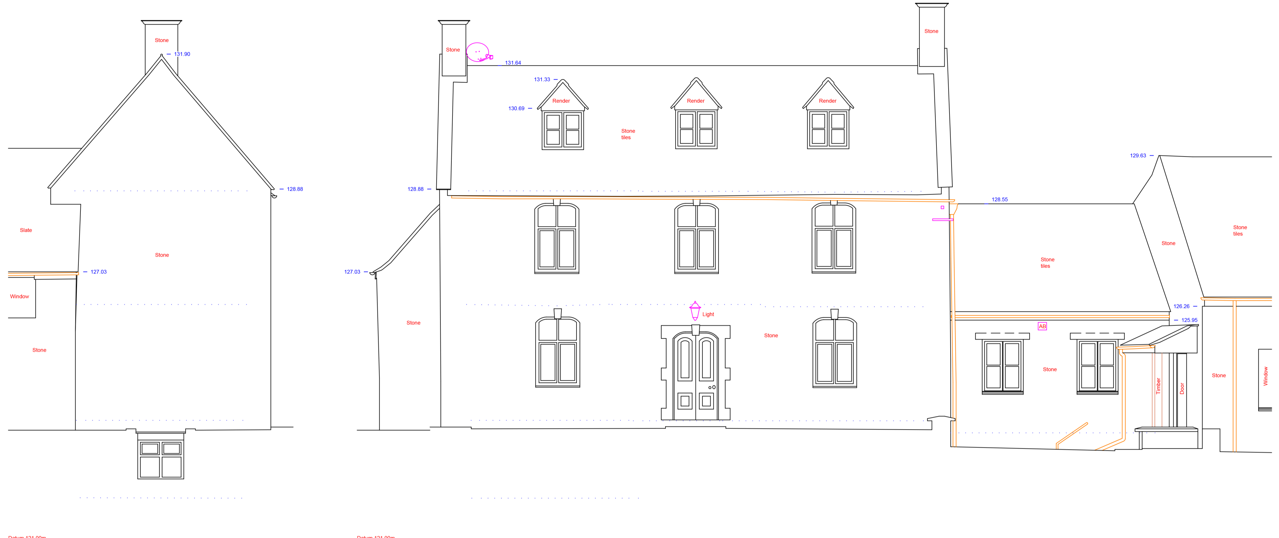
SOUTH WEST ELEVATION
