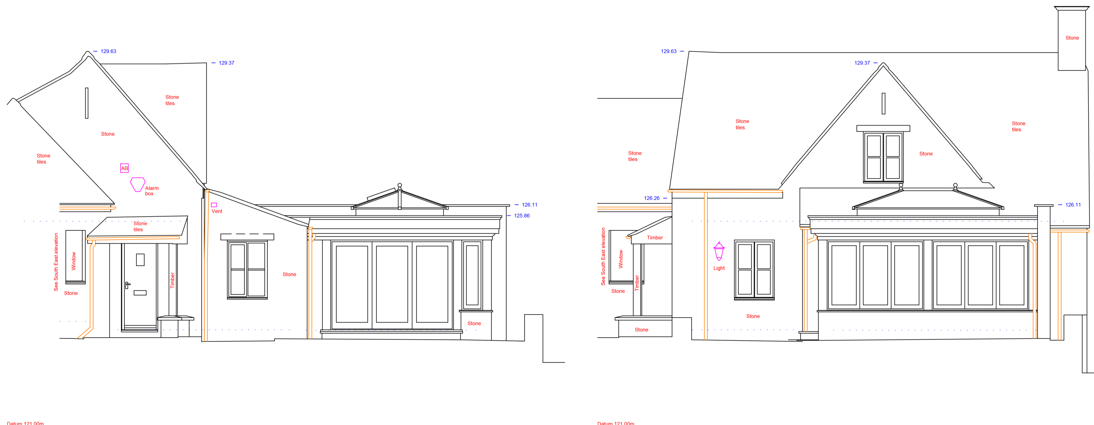
SOUTH ELEVATION
