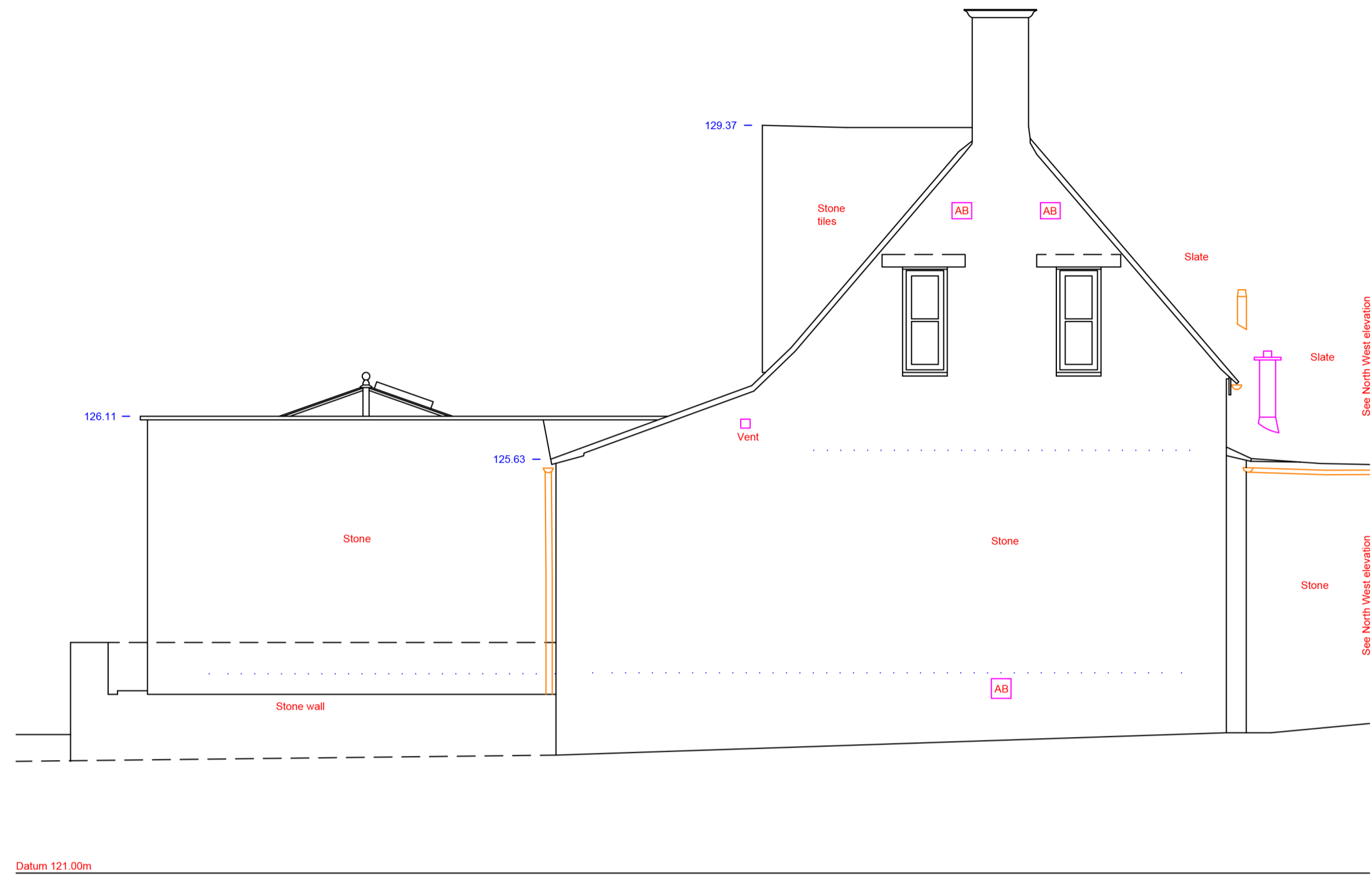
NORTH ELEVATION
