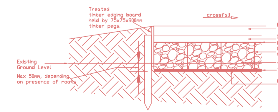
CONSTRUCTION DETAIL FOR NO-DIG AREA
