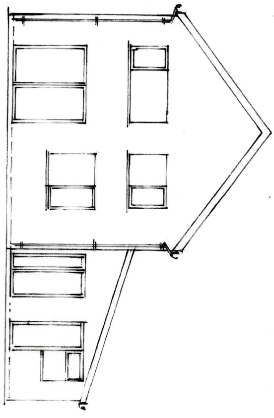
EXIST REAR ELEVATION. E.
