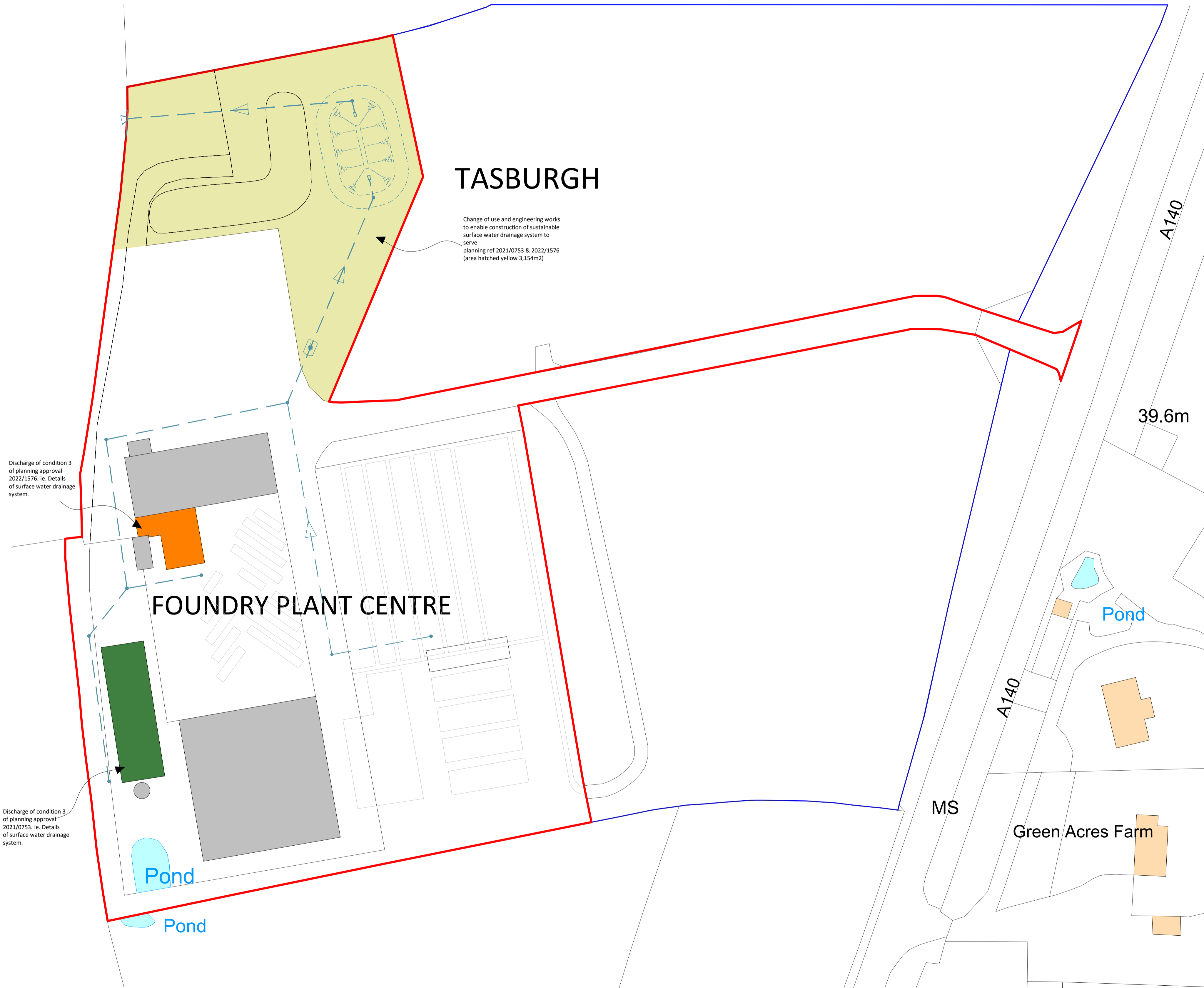
BLOCK PLAN
