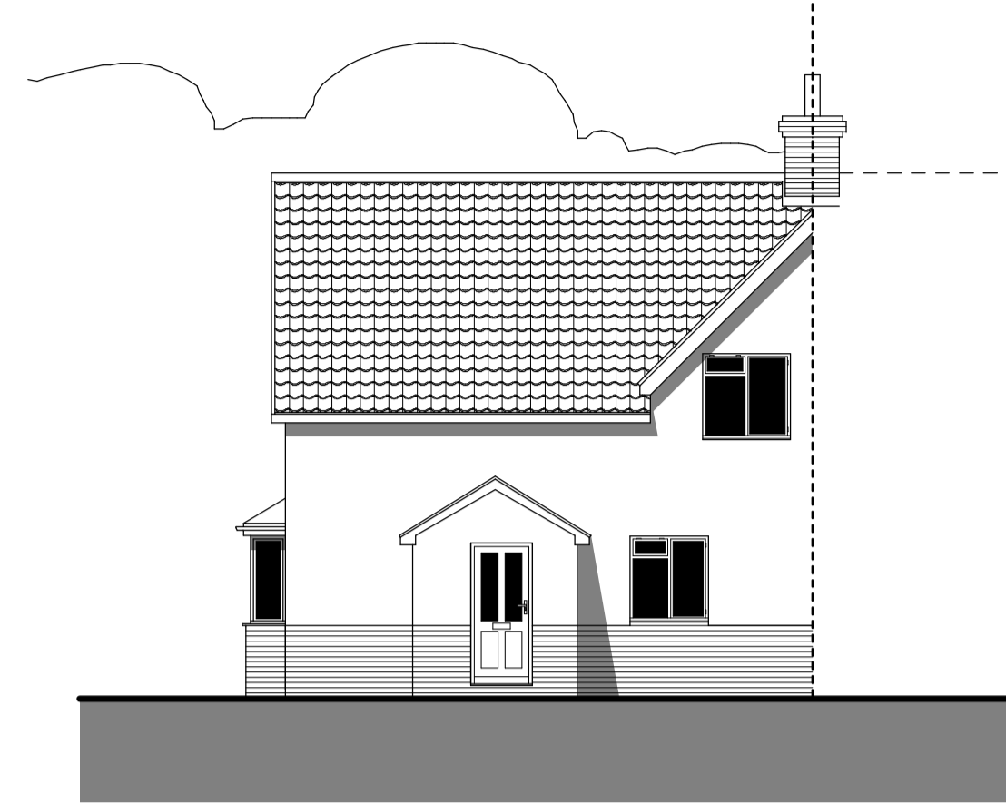
South Elevation
