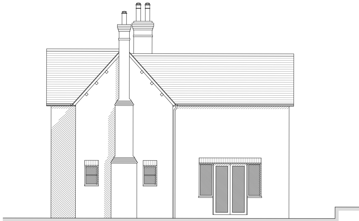
EXISTING NORTH-WEST ELEVATION
