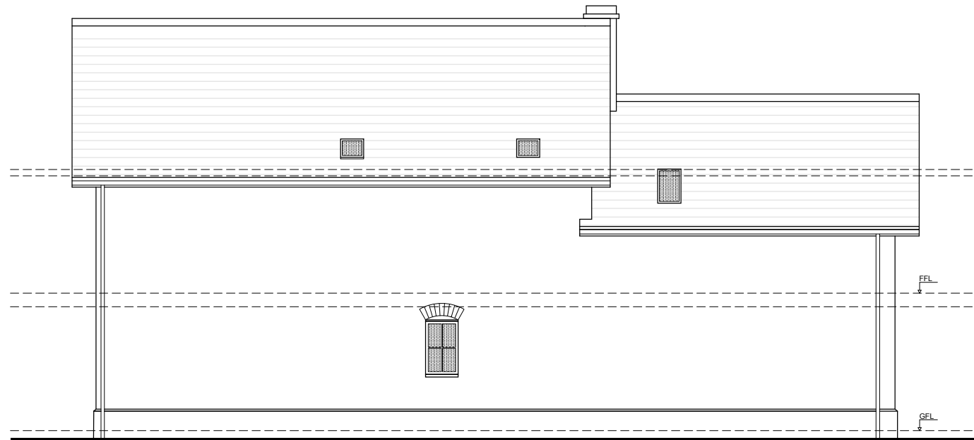
④ Existing South (Side) Elevation. 1:100
