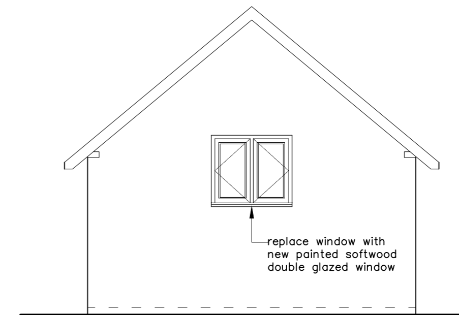
North elevation
