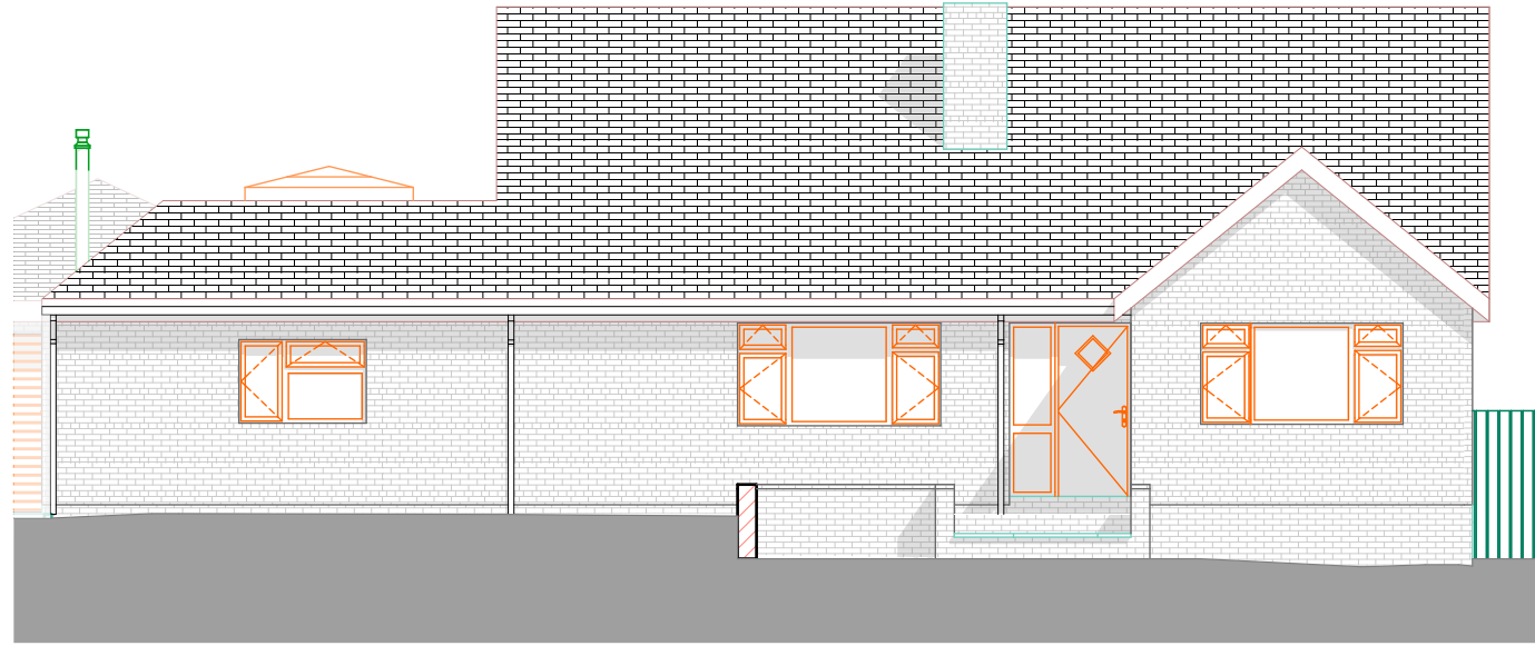
East Elevation
