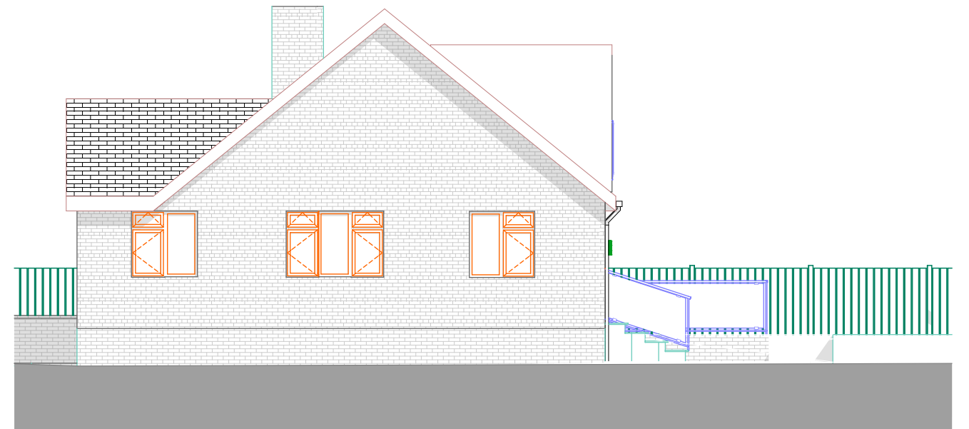
North Elevation
