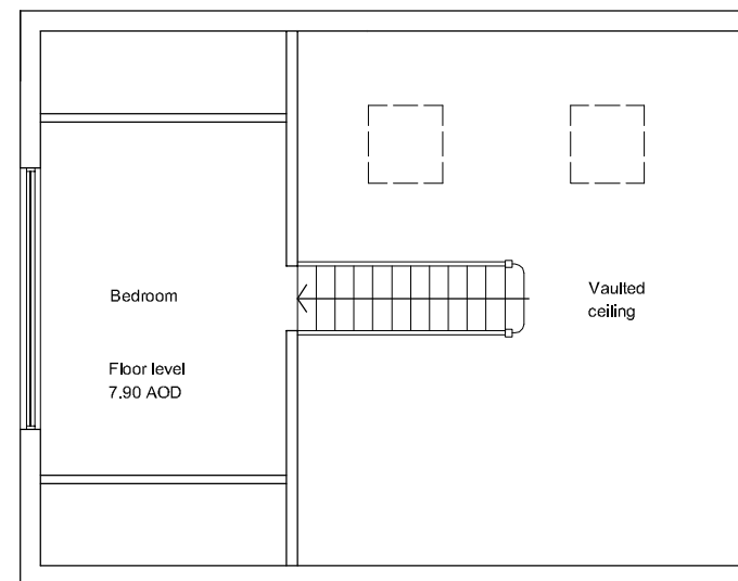
PROPOSED FIRST FLOOR PLAN 1:100
