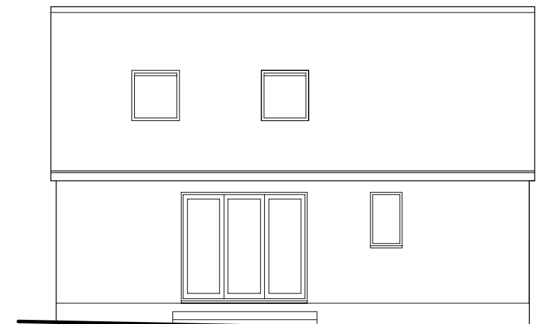
PROPOSED NORTH-WEST ELEVATION 1:100
