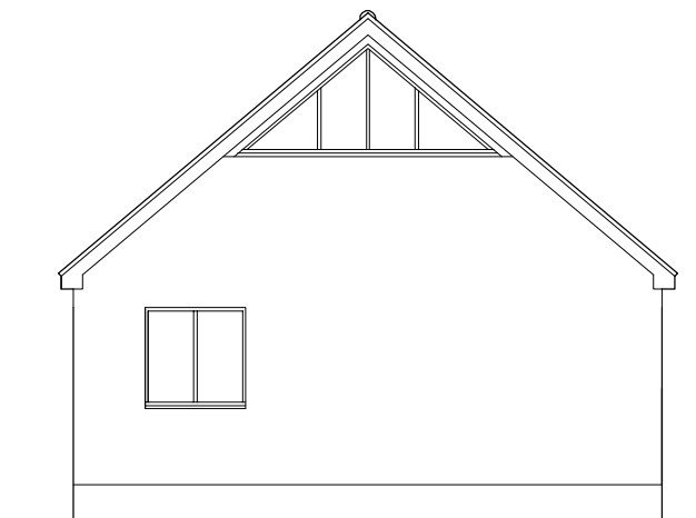
PROPOSED REAR ELEVATION 1:100
