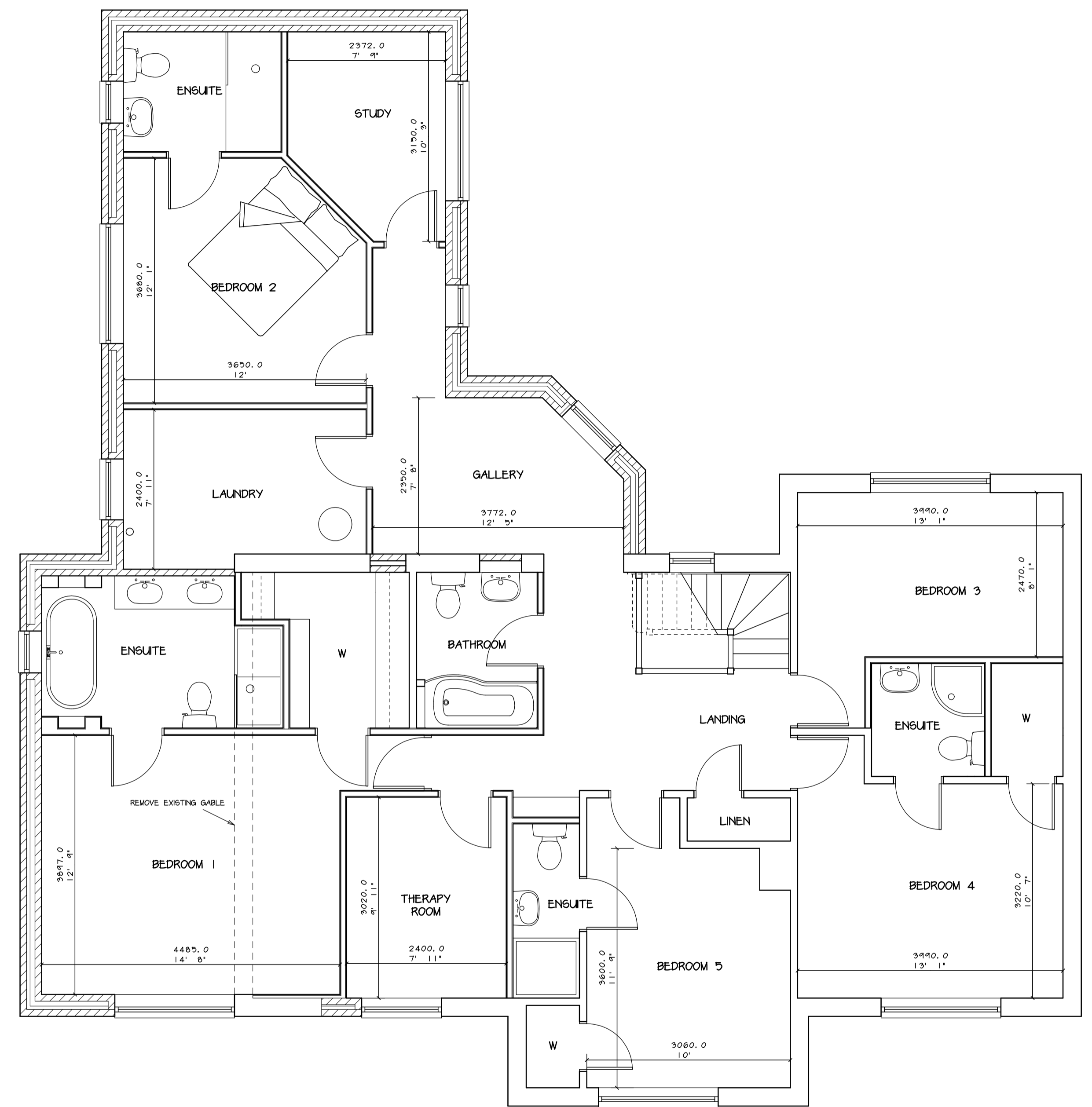
FIRST FLOOR
