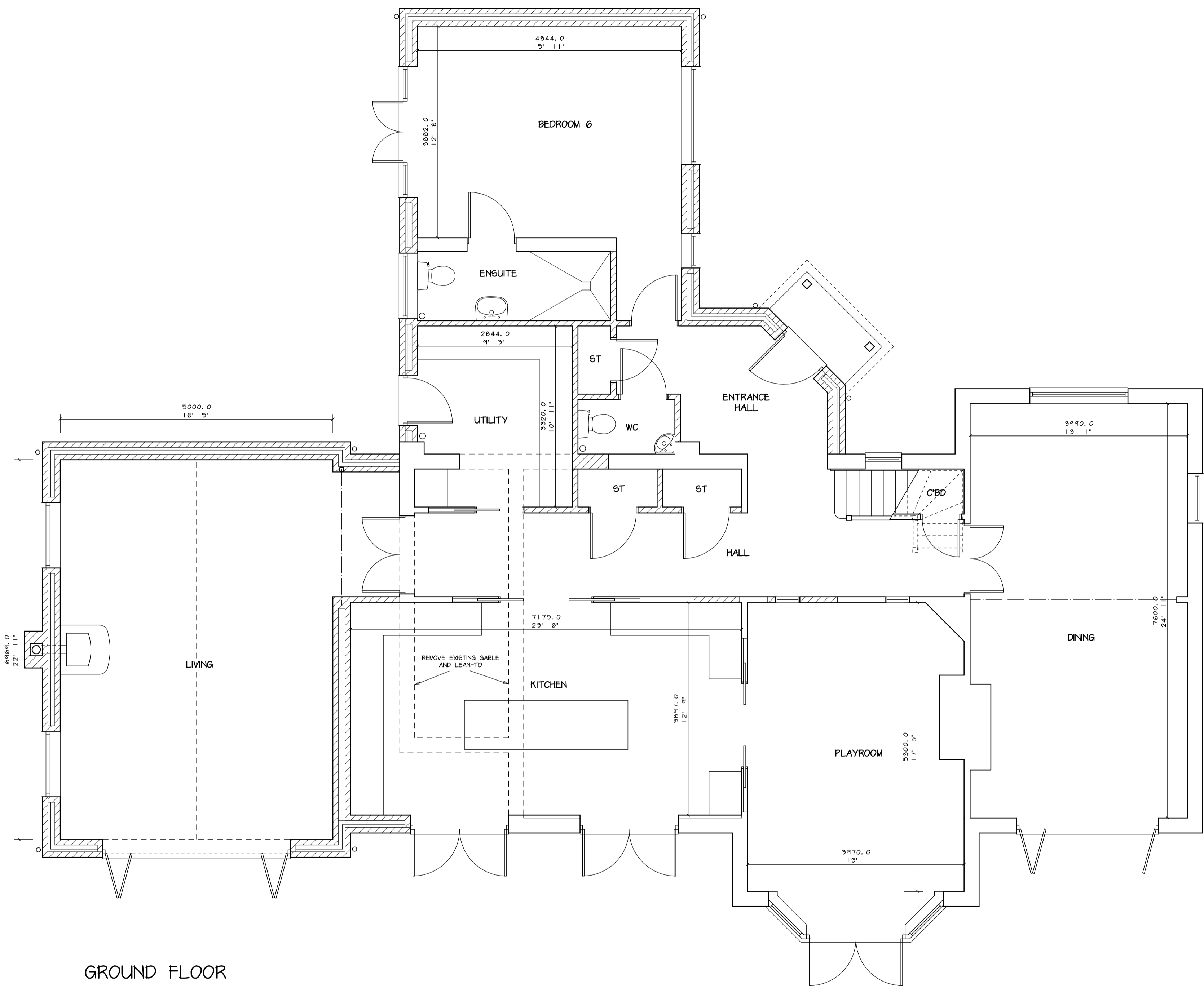
PROPOSED LAYOUTS
