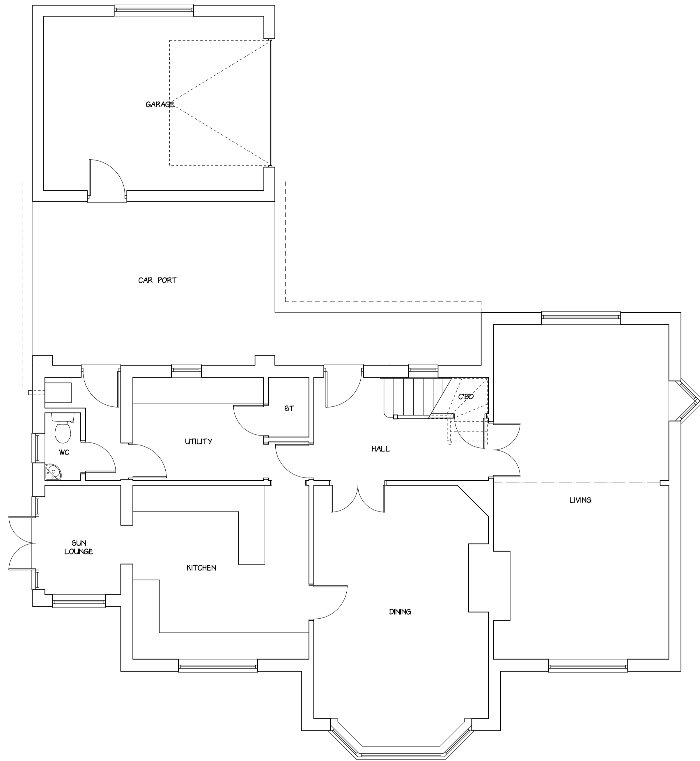
GROUND FLOOR
