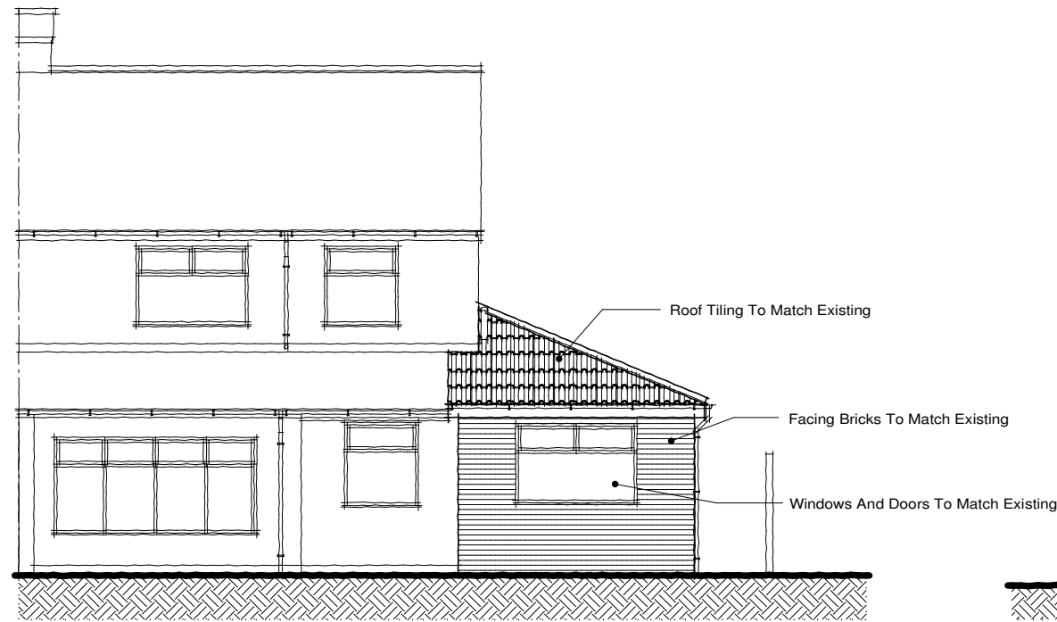
Front Elevation
