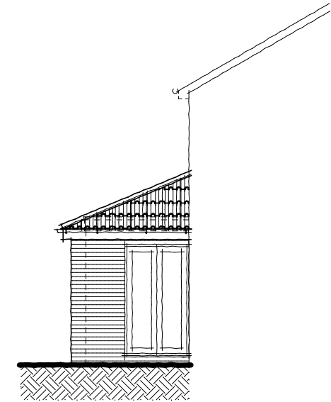
Side Elevation
