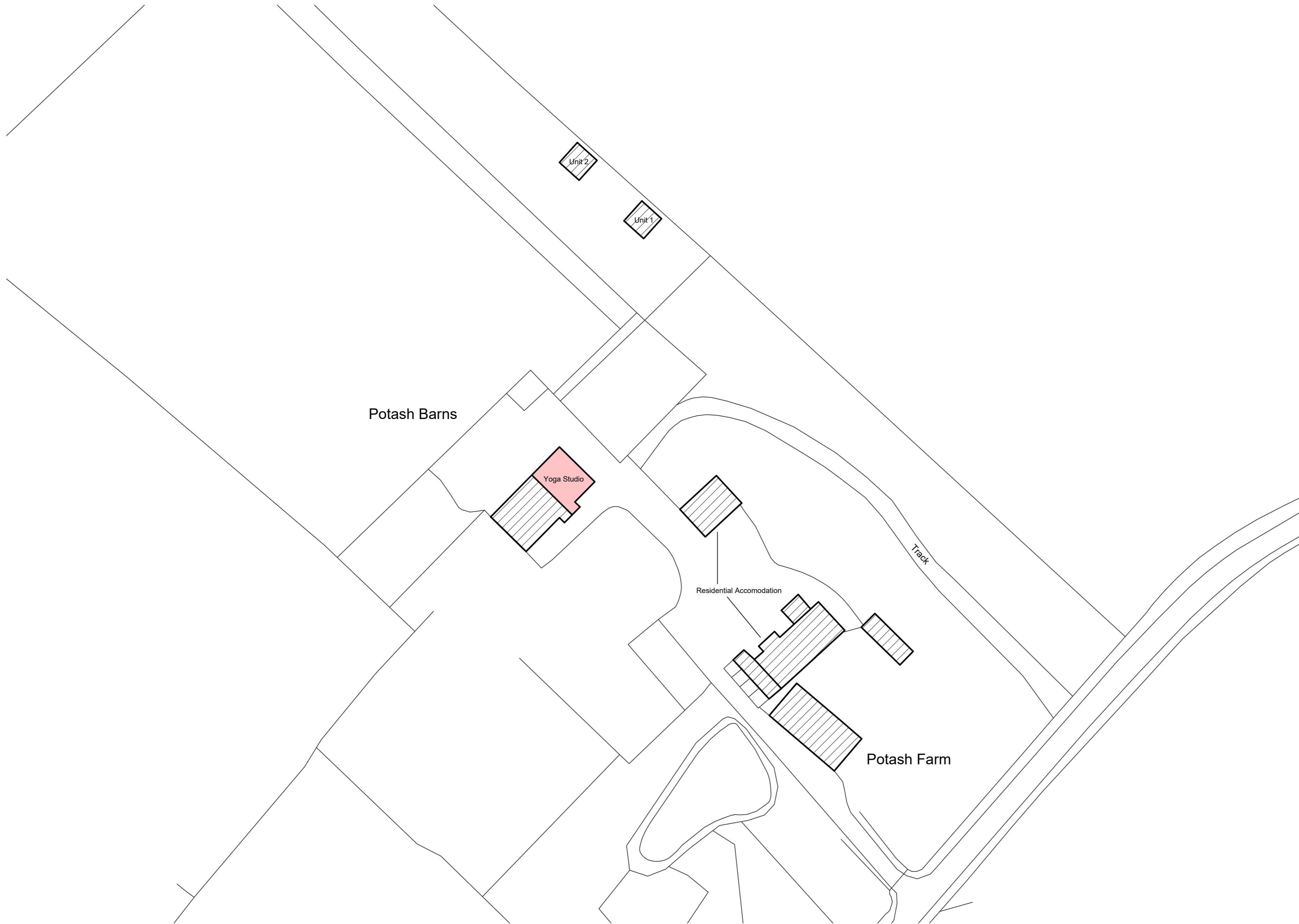
Existing Block Plan - 1:500
