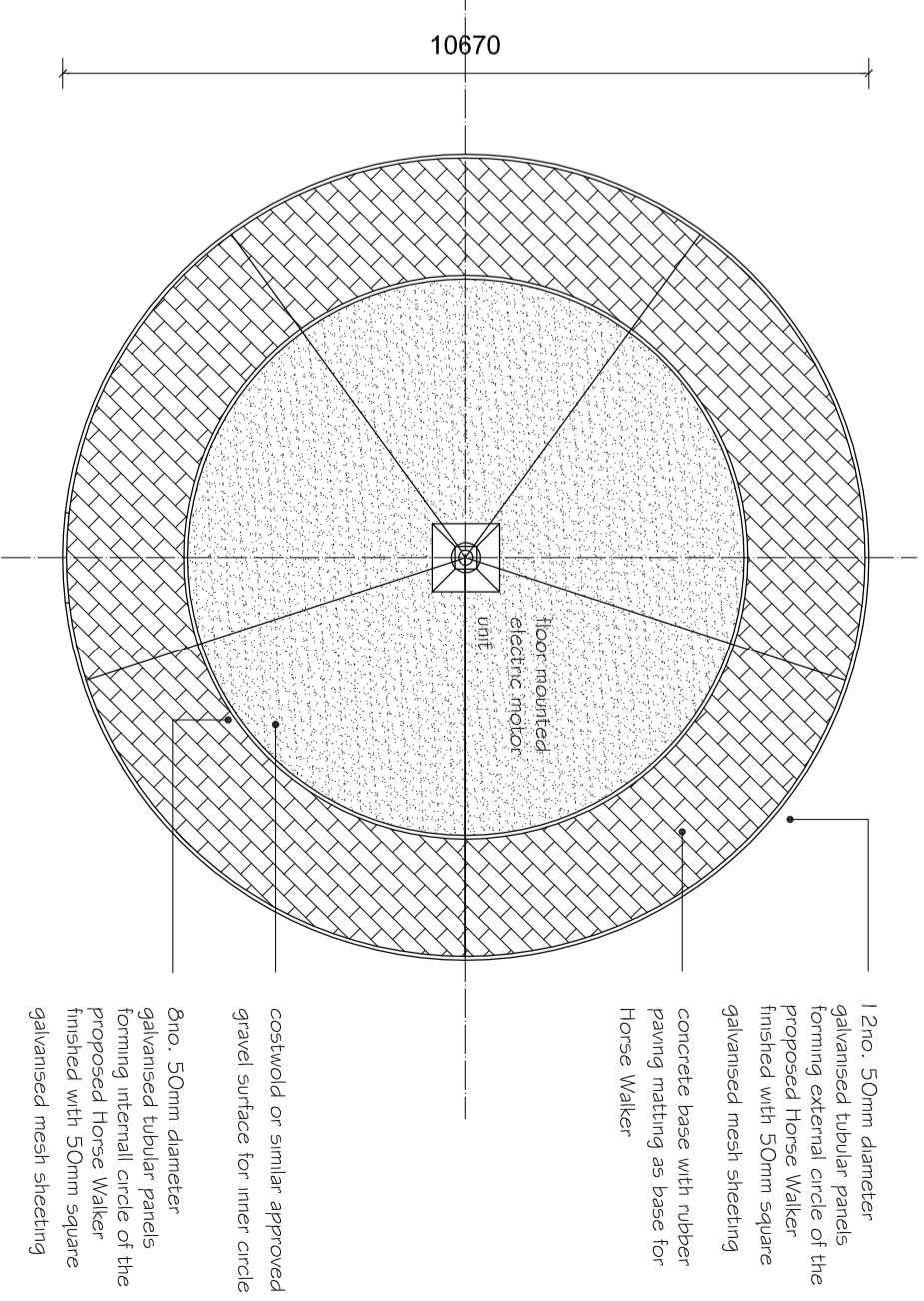
H O R S E W A L K E R P L A N Scale 1:100
