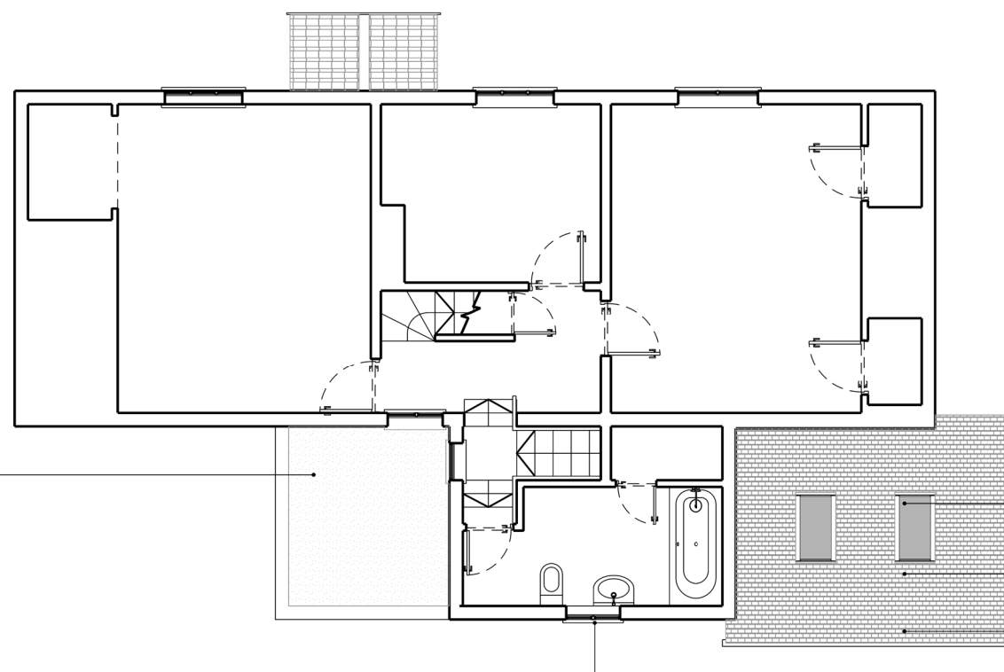
Proposed - Plan - 01 1:100
