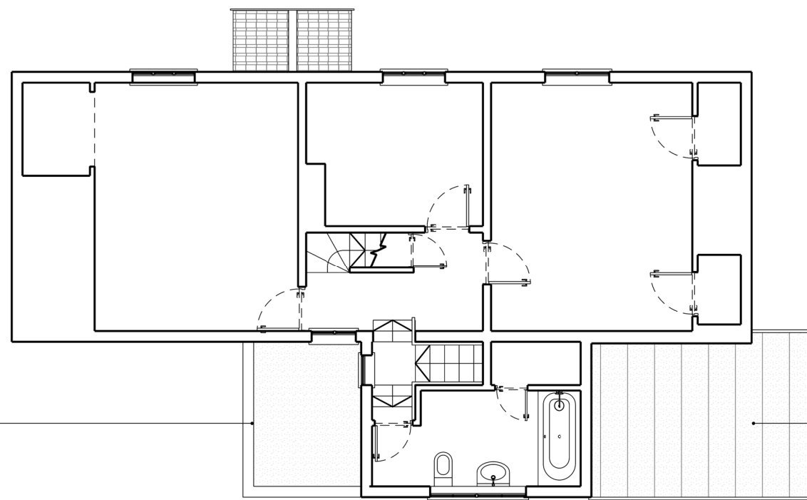
Existing - Plan - 01 1:100
