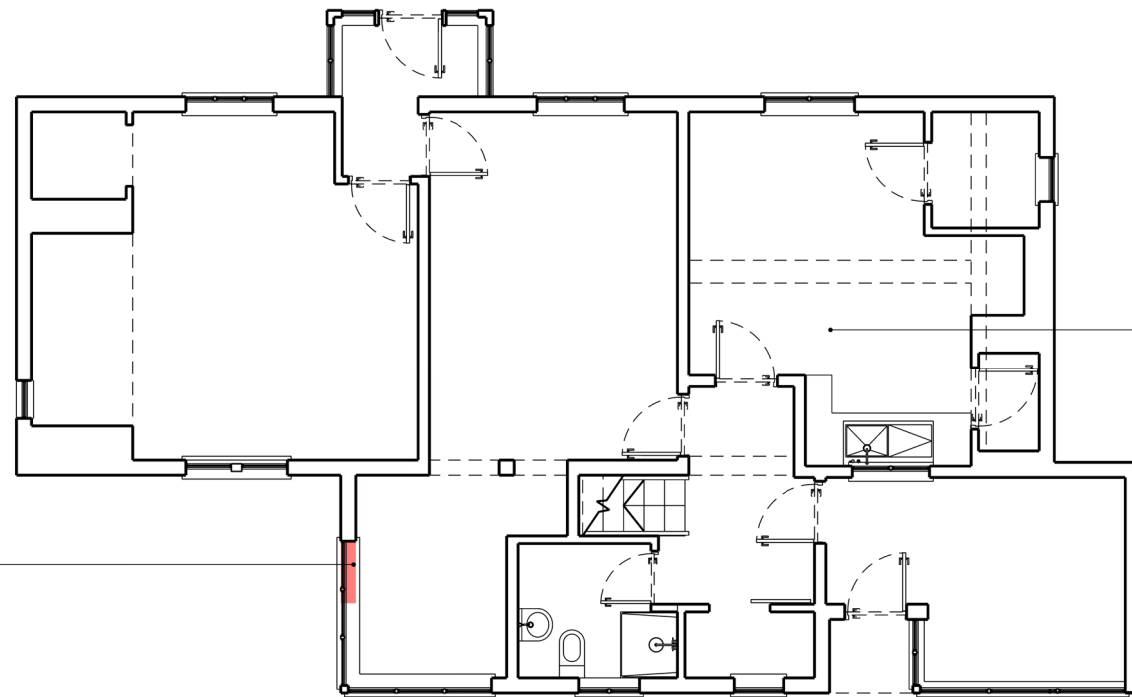
Existing - Plan - 00 1:100
