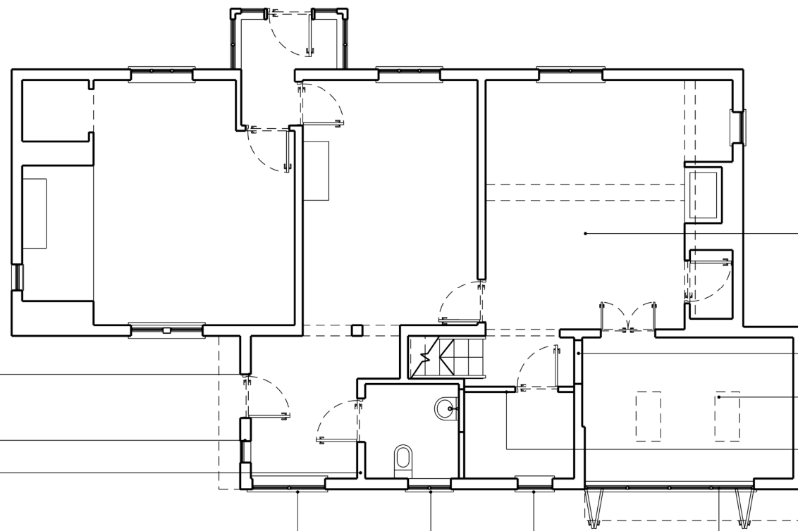
Proposed - Plan - 00 1:100
