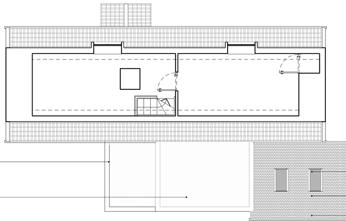
Proposed - Plan - 02 1:100
