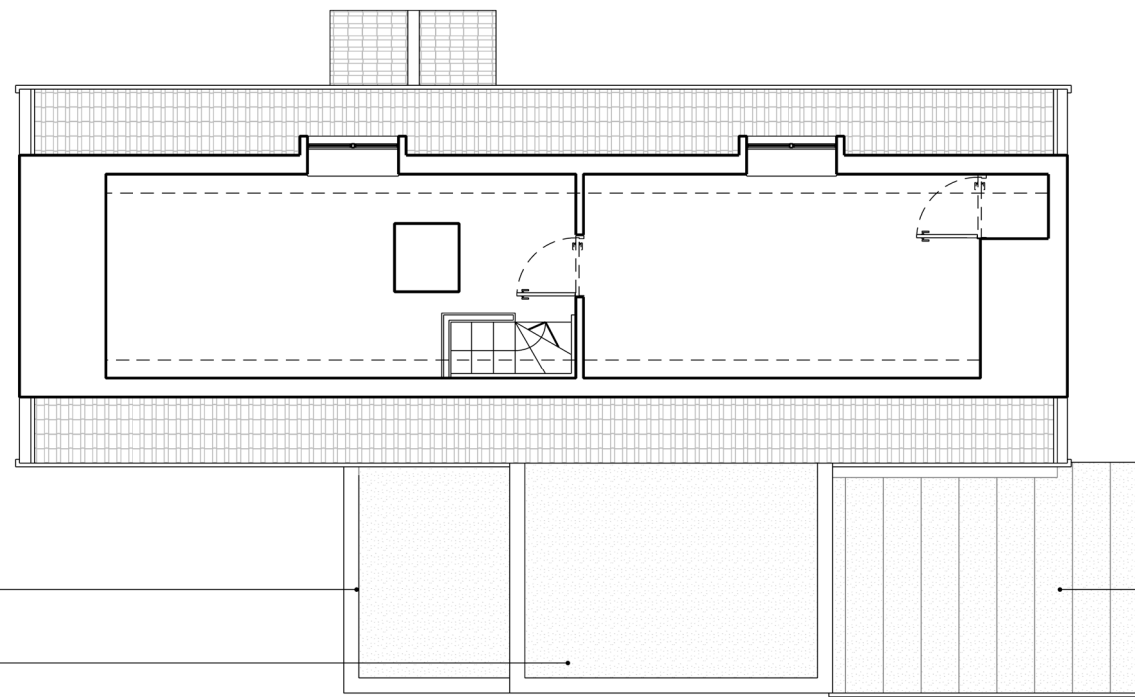
Existing - Plan - 02 1:100
