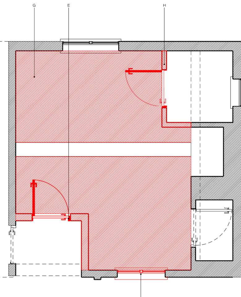
IRL - Existing - Reflected Ceiling Plan - Kitchen 1:50
