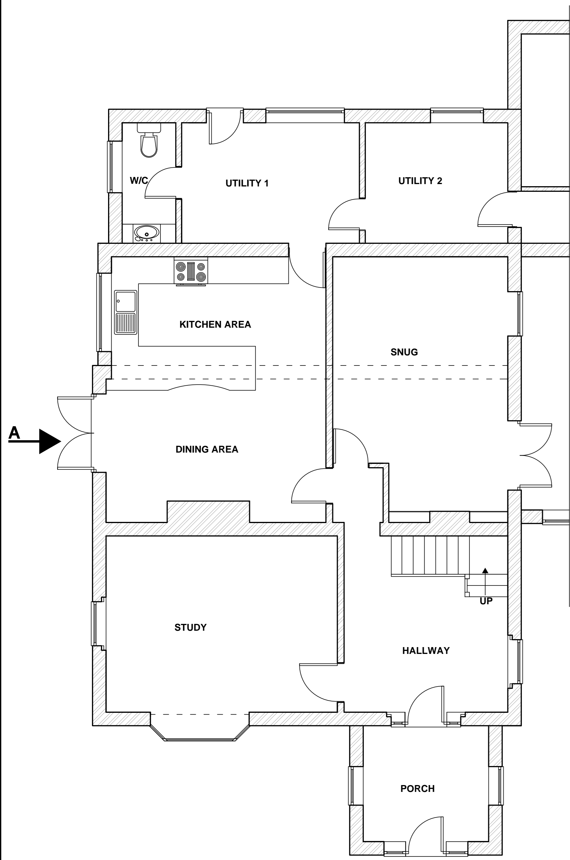
AS EXISTING GROUND FLOOR PLAN - 1:50
