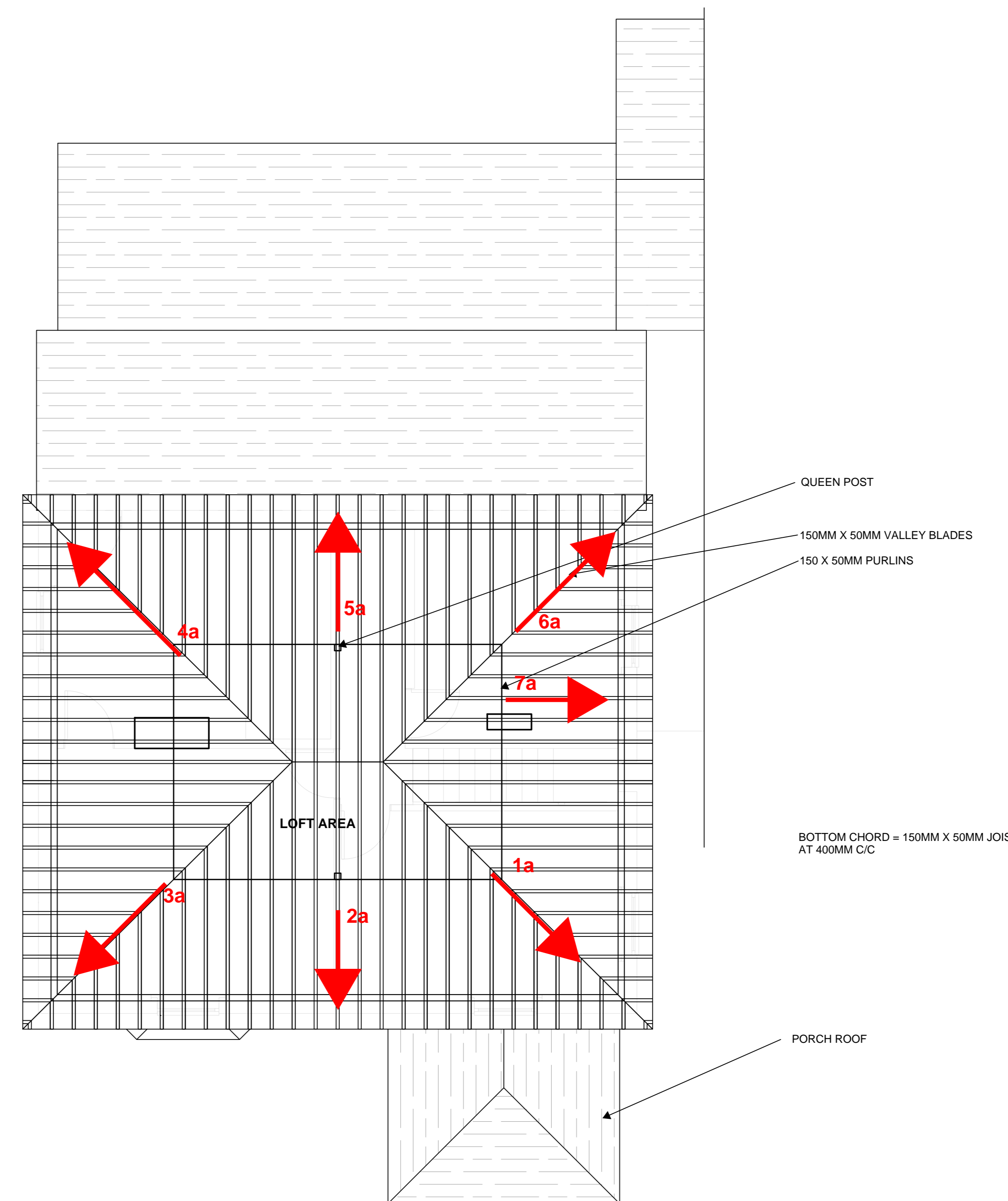
AS EXISTING LOFT FLOOR PLAN - 1:50
