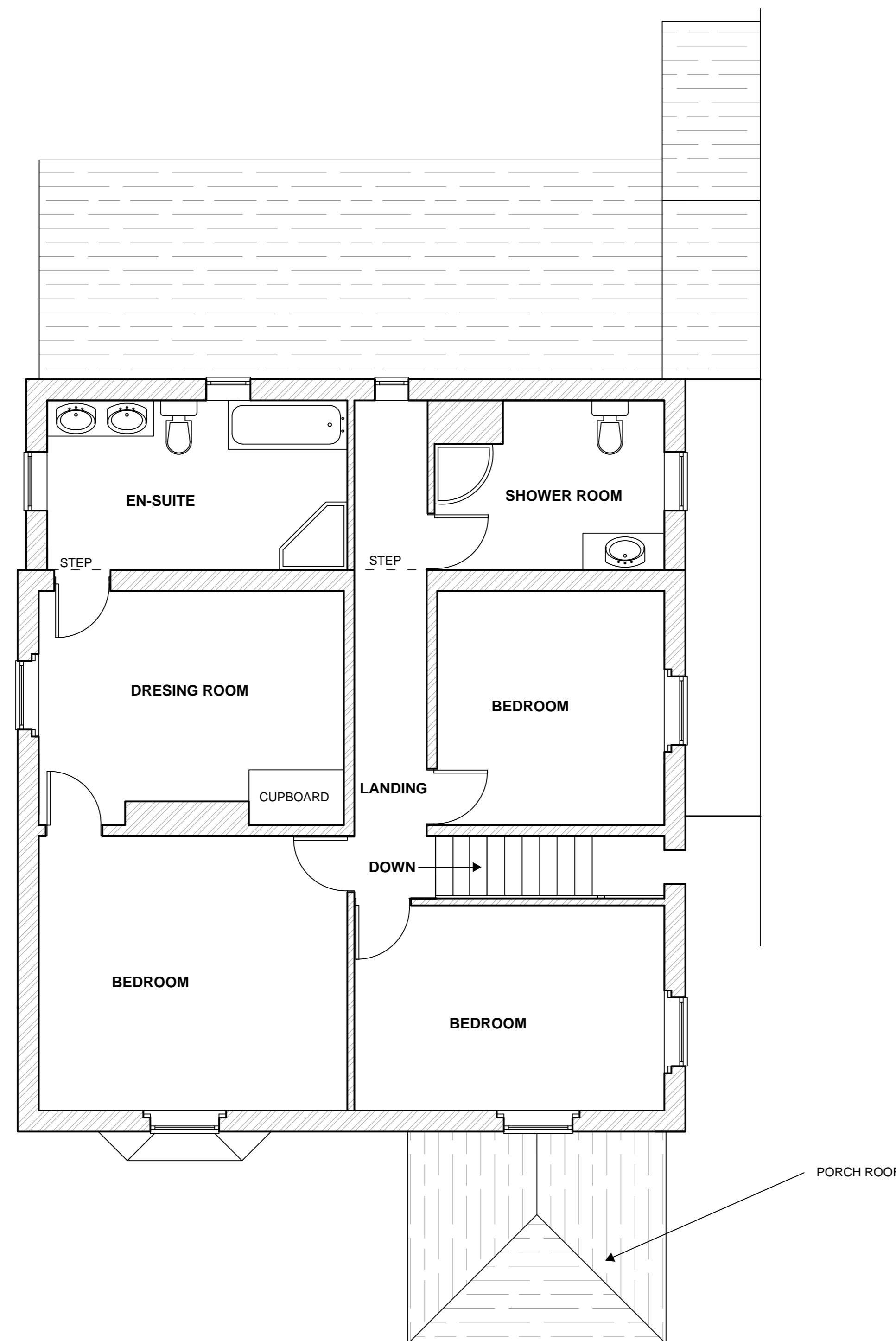
AS EXISTING FIRST FLOOR PLAN - 1:50
