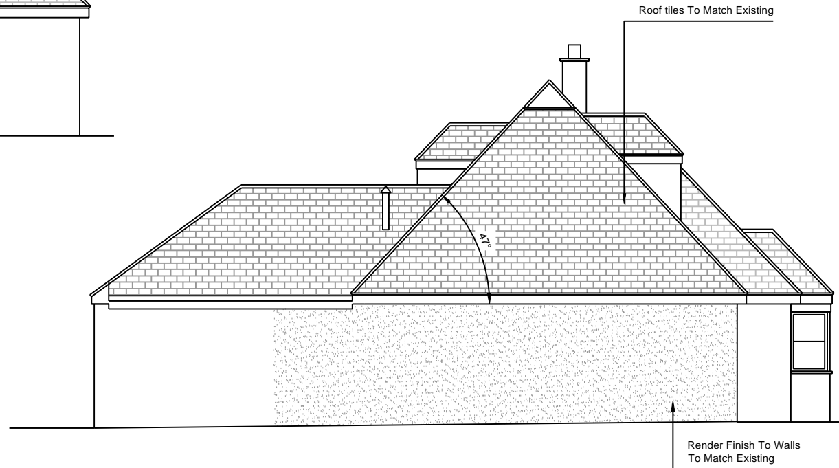
LEFT ELEVATION
