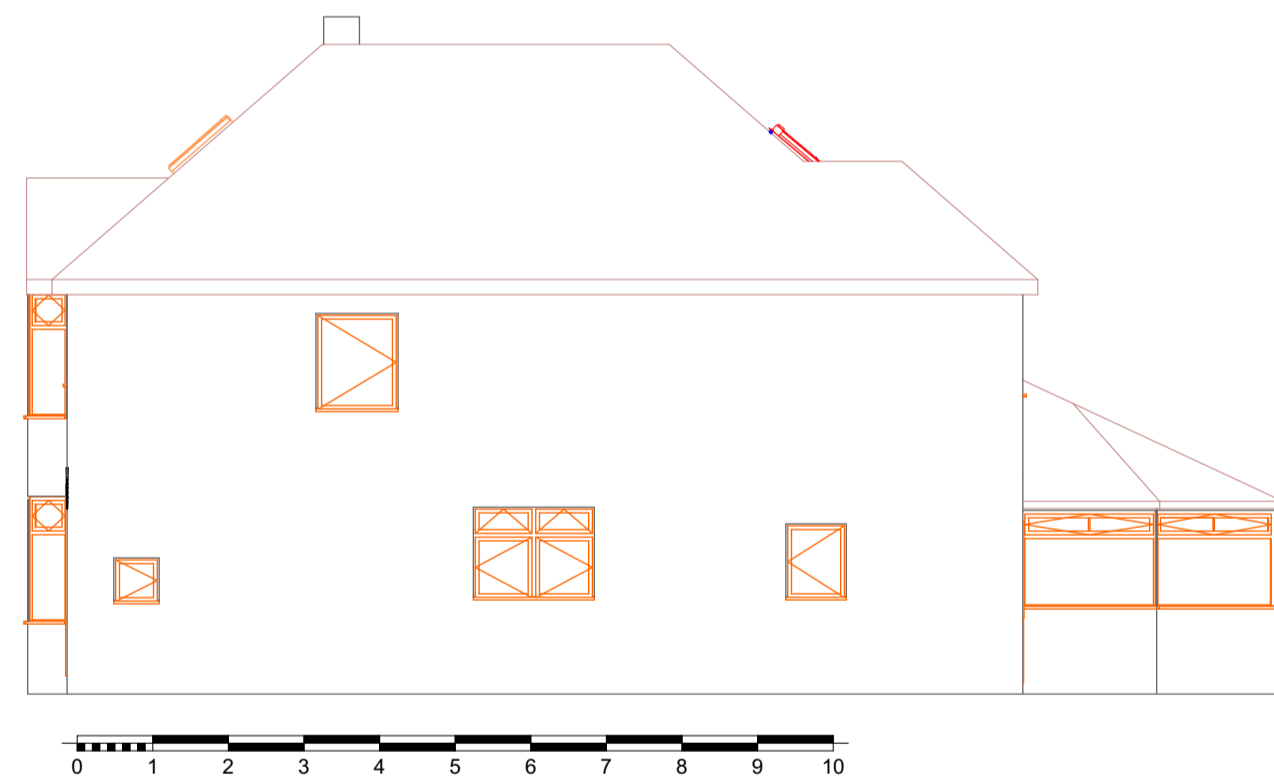
3 East Elevation Existing 1:100
