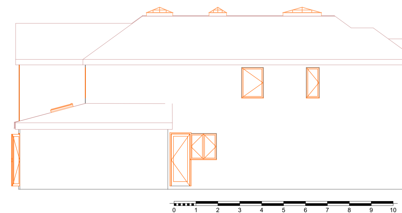
8 West Elevation Proposed 1:100
