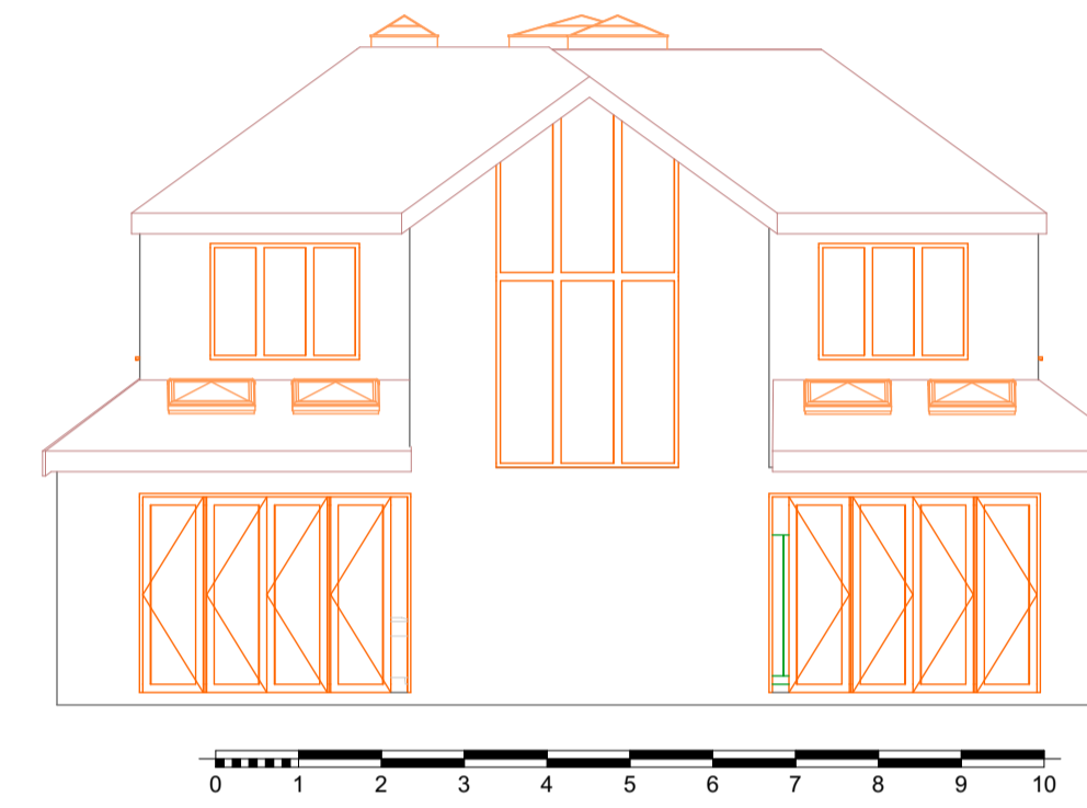
6 North Elevation Proposed 1:100
