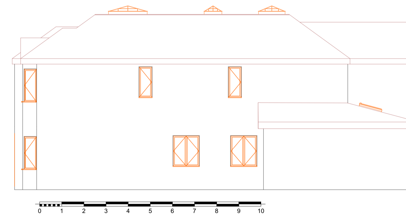
7 East Elevation Proposed 1:100
