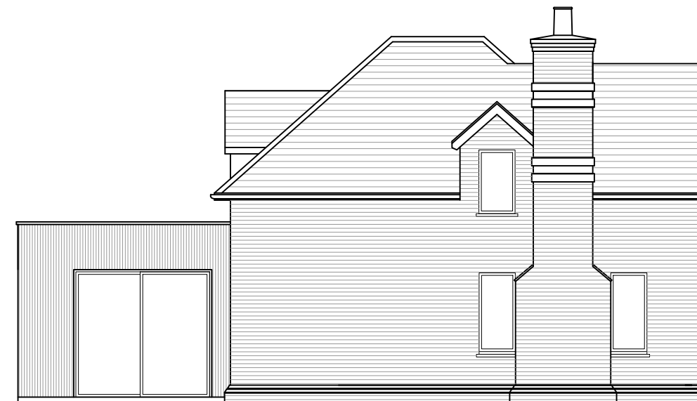
PROPOSED RIGHT NORTH SIDE ELEVATION
