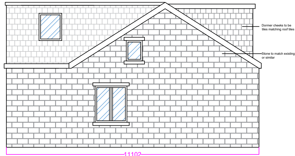
PROPOSED RIGHT SIDE ELEVATION
