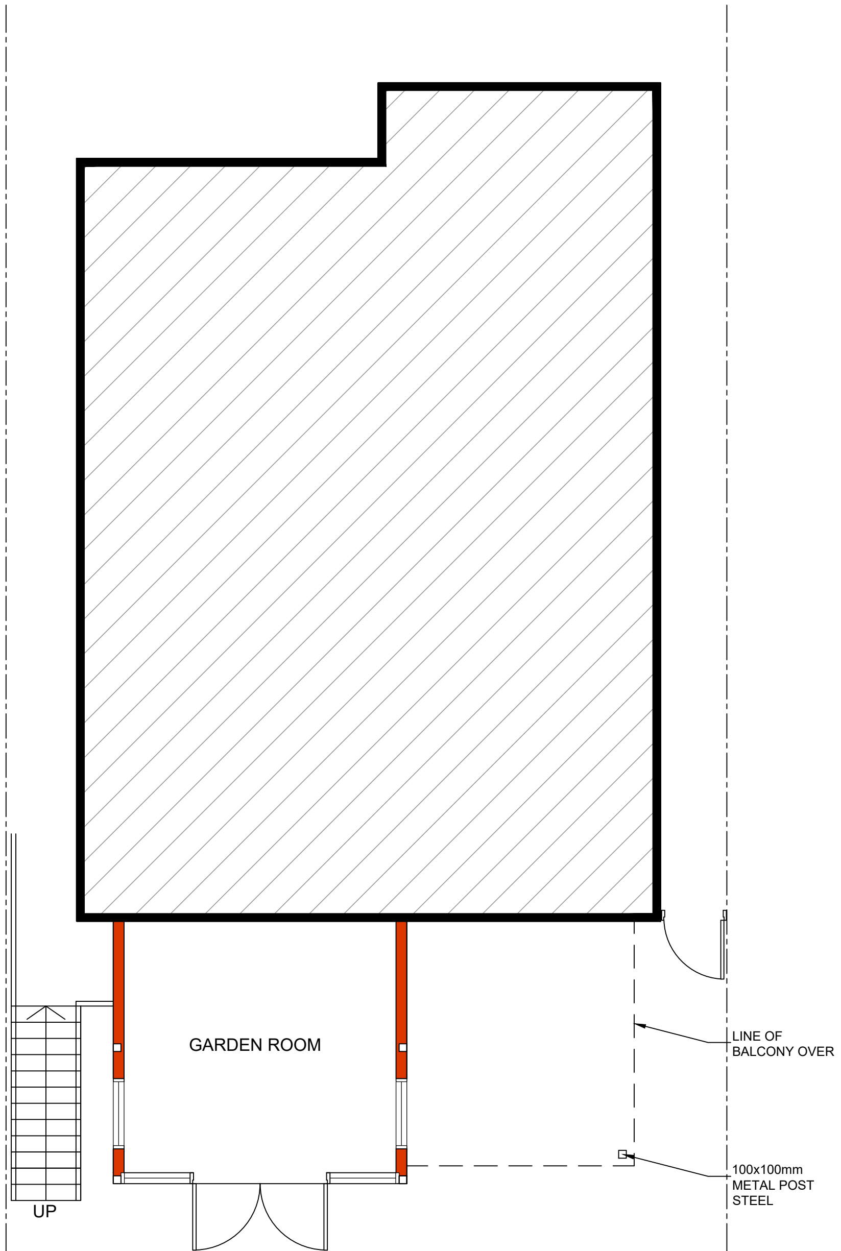
LOWER GROUND FLOOR PLAN AS PROPOSED
