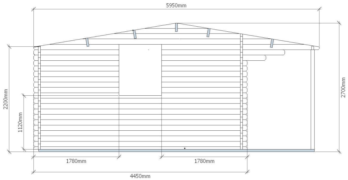
NW side elevation
