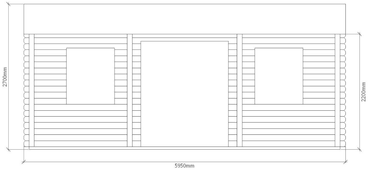
Front SW elevation detail
