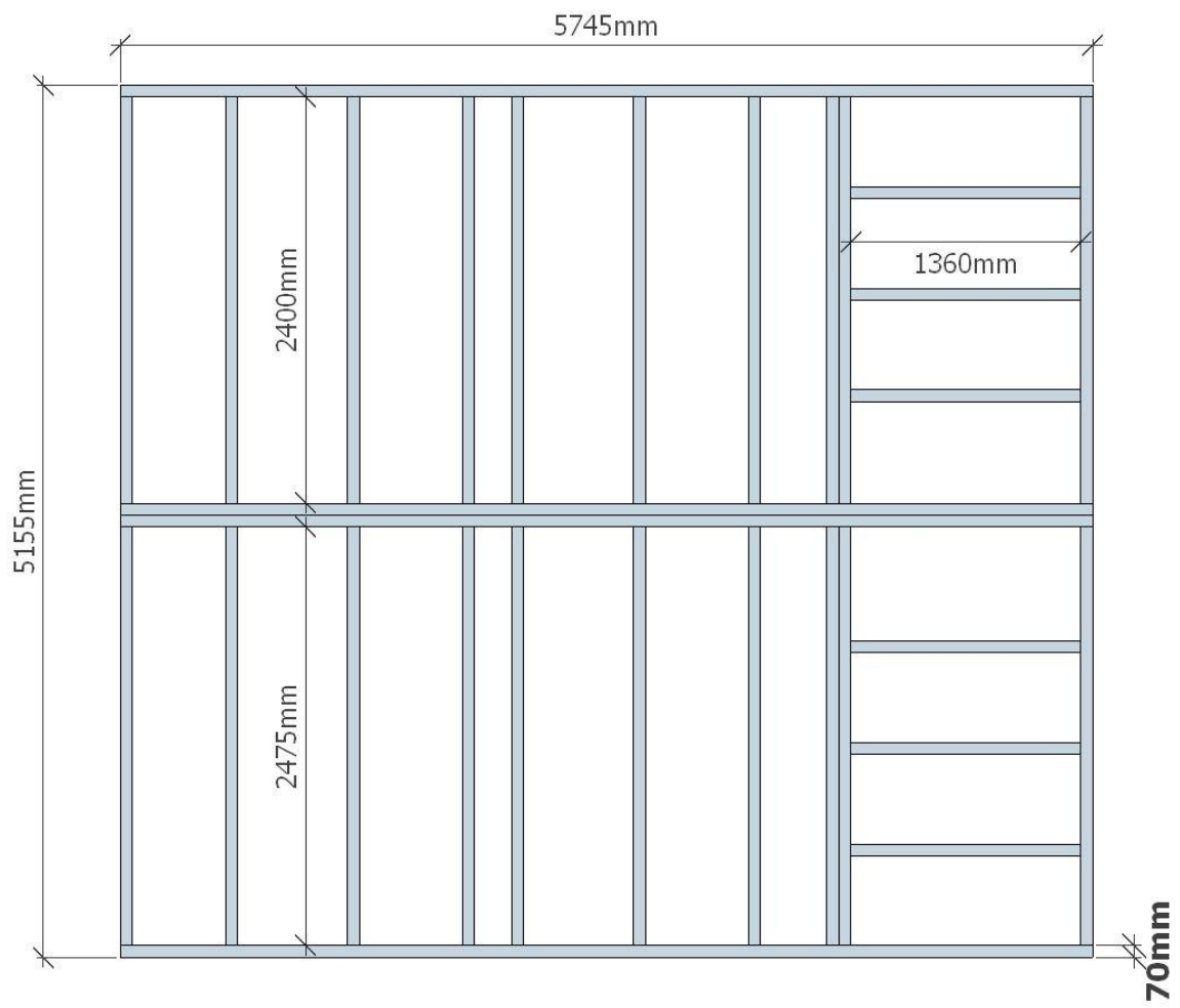
Floor frame
