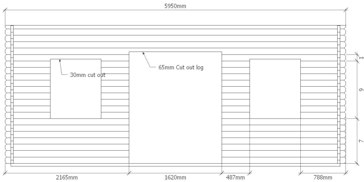
Front SW elevation detail
