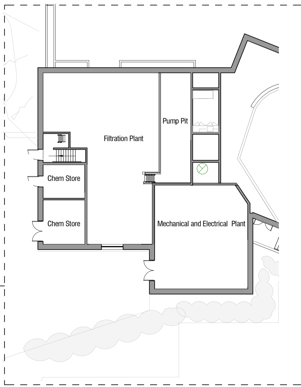
Level 1 Plant GA Plan
