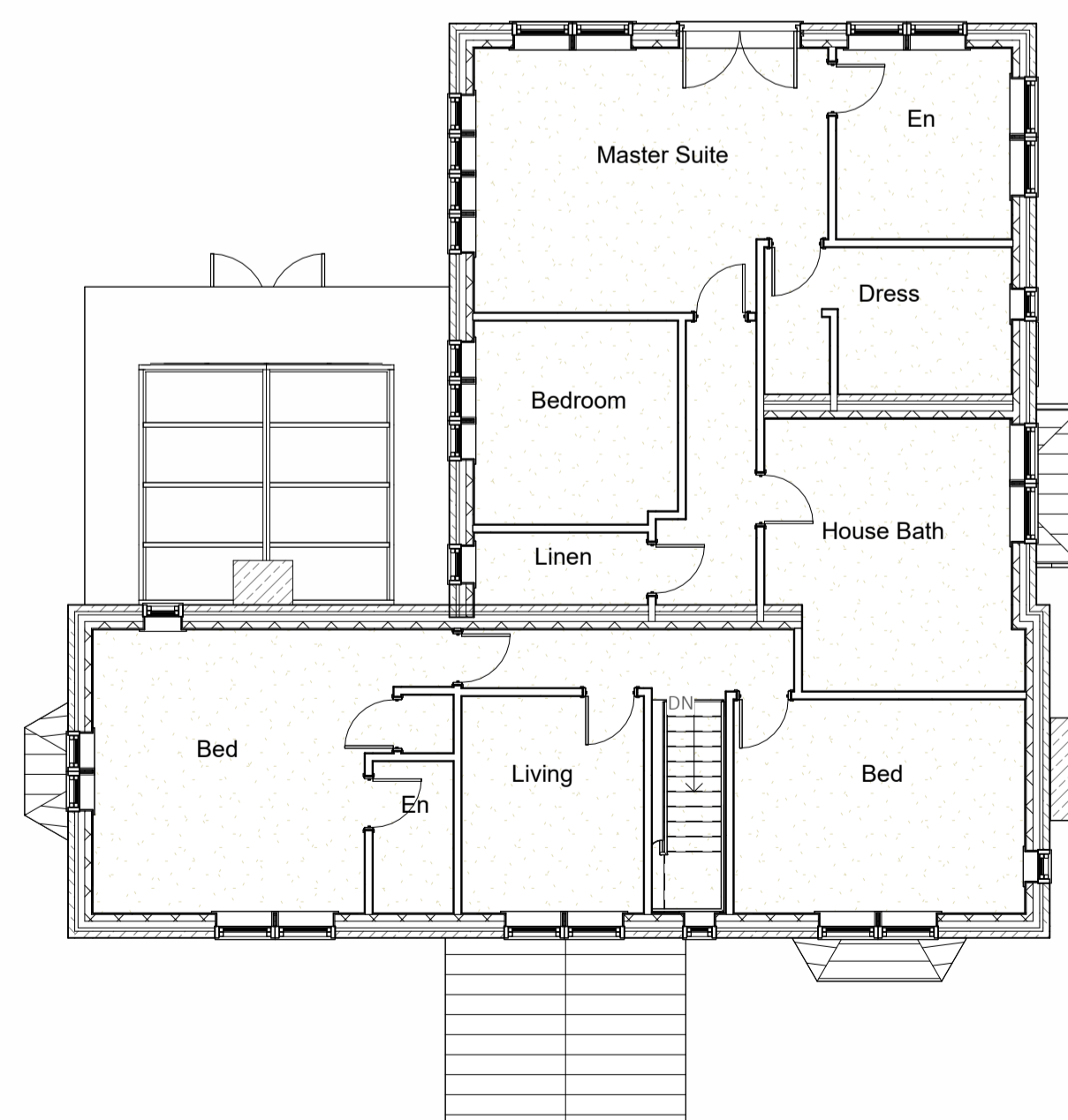
2 First Floor 1 : 100
