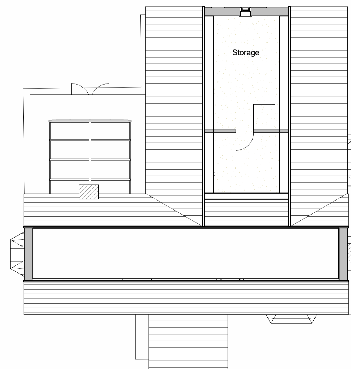
7 Second Floor 1 : 100
