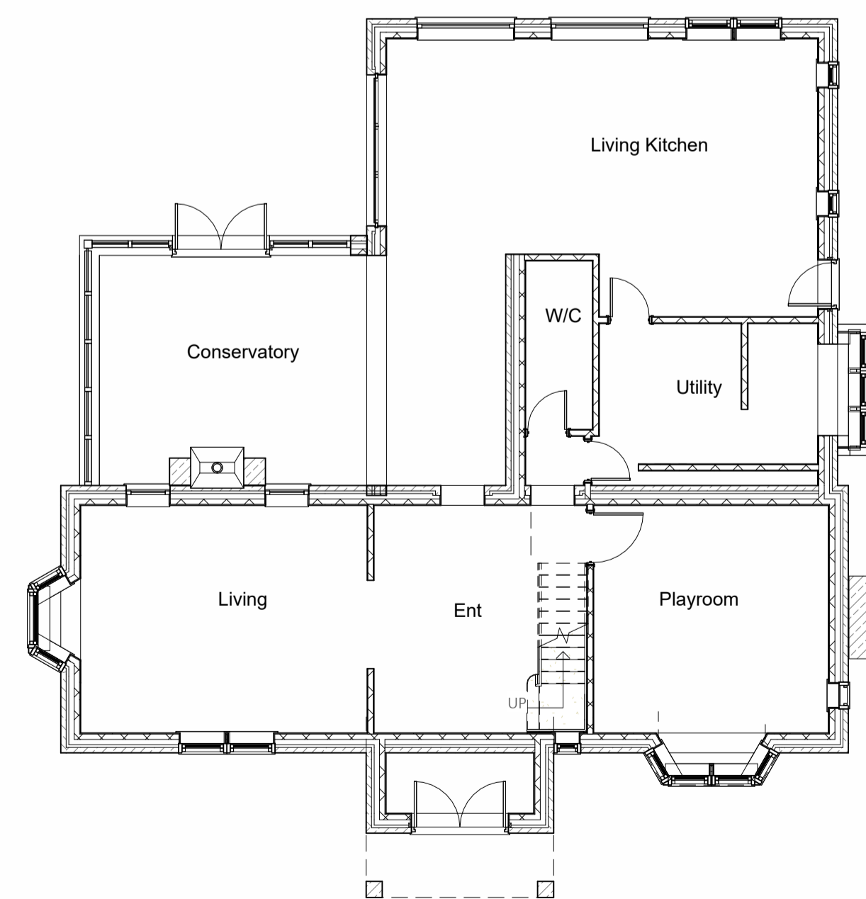
1 Ground Floor 1 : 100
