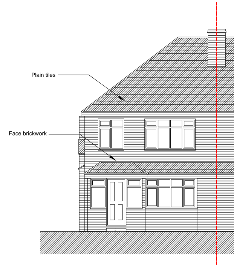
Front Elevation...
