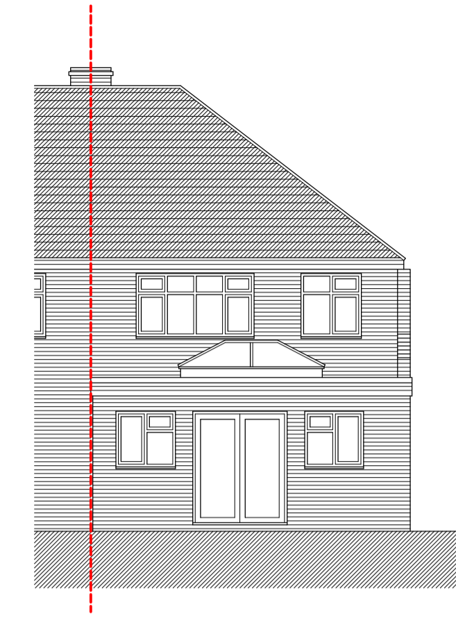
Rear Elevation...
