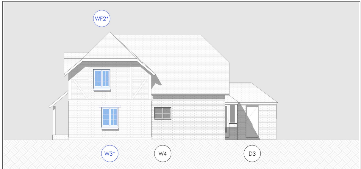
Figure 2 – South (Side) Elevation Elevation
