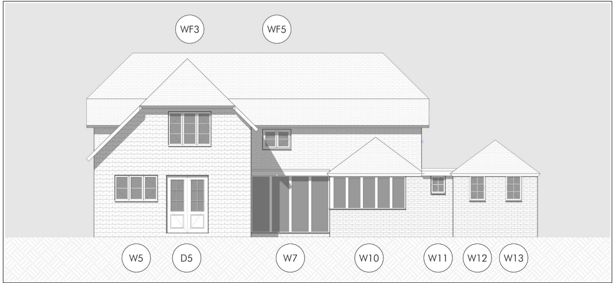
Figure 3 – East (Rear) Elevation
