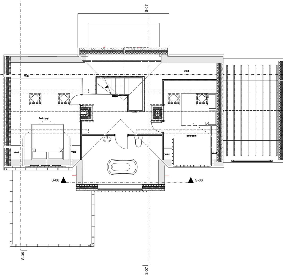
Proposed Attic Floor Plan
