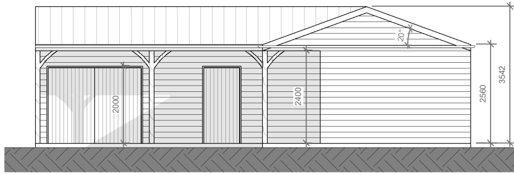
Rear Elevation
