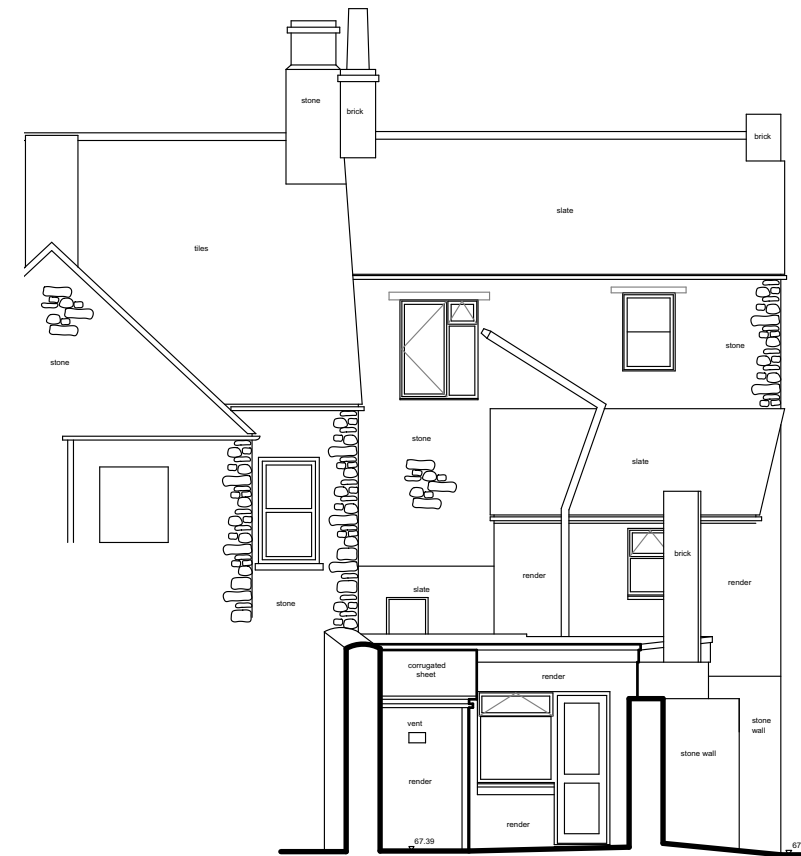
2 Existing north elevation Scale: 1:100
