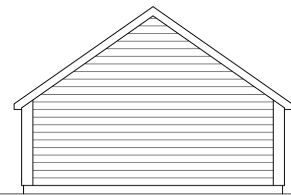
North-East Elevation
