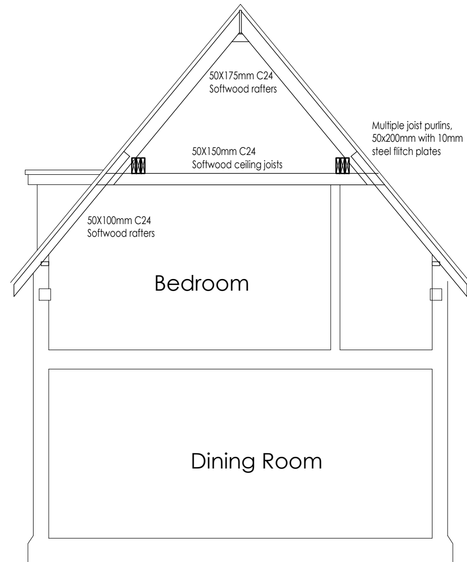
PROPOSED SECTION
