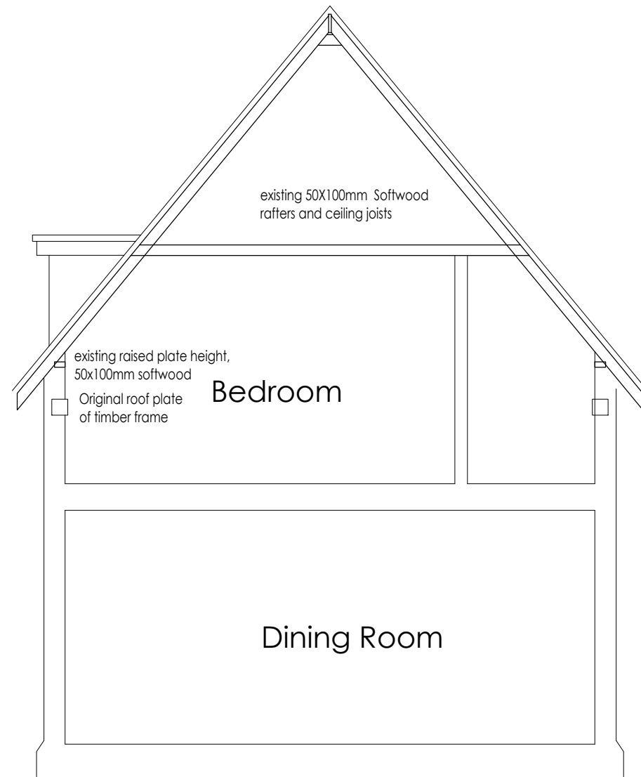
EXISTING SECTION
